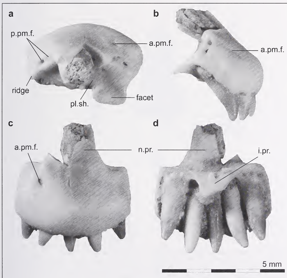
FIG. 1. Partial premaxilla of Tinosaurus sp. MPH, PTRM 19515, in (a) dorsal, (b) right lateral, (c) anterodorsal, and (d) posteroventral views. Abbreviations: a.p.m.f., anterior premaxillary foramen; i.pr., incisive process; n.pr., nasal process; pl.sh., palatal shelf; p.p.m.f., posterior premaxillary foramen.
