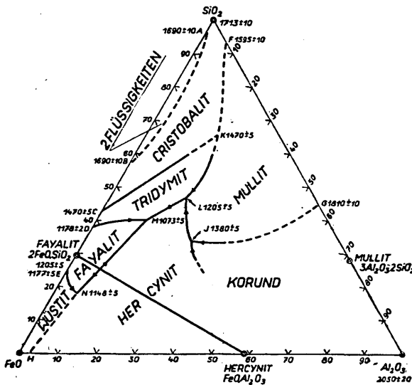
Abb. 5, System FeO—Al 2 O 3 —SiO 2
