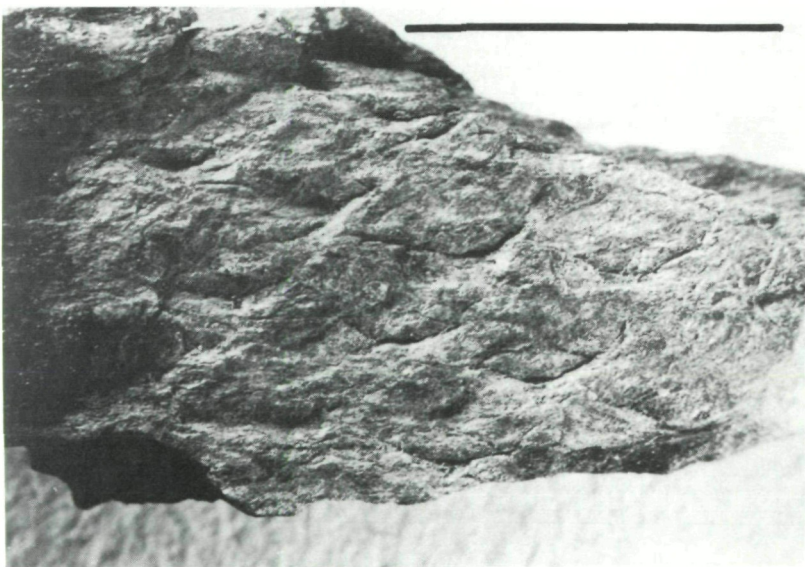
Abb. 5: Lepidofloyos sp.
