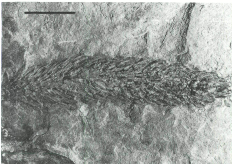
Abb. 2: Palaeostachya sp.
