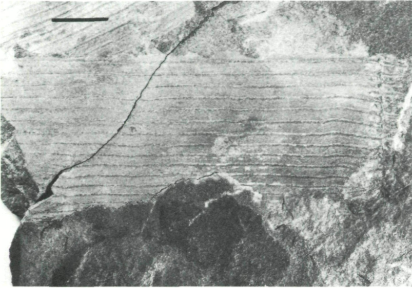
Abb. 2: Calamites sp.
