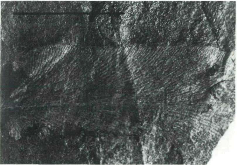
Abb. 14: Linopteris sp.
