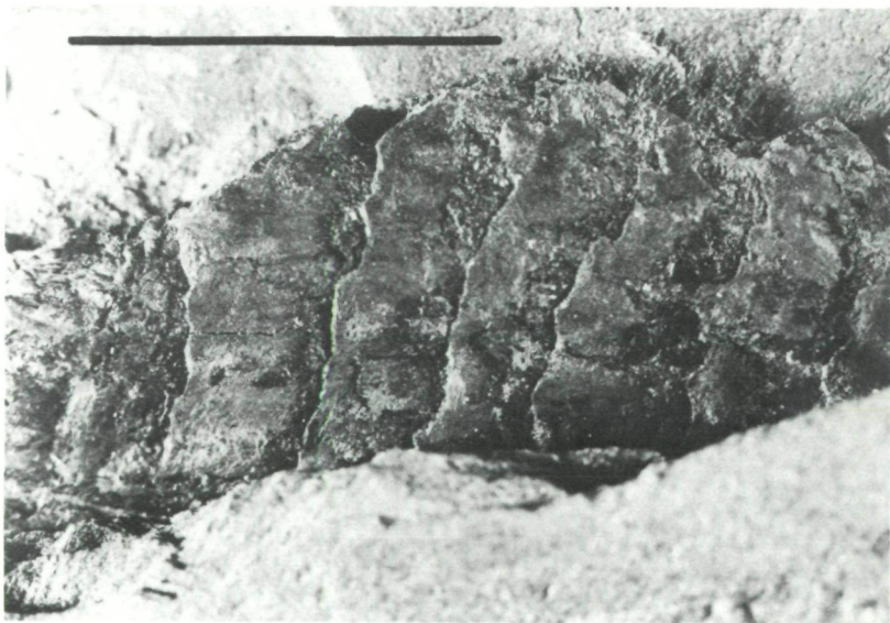
Abb. 3: Macrostachya sp.
