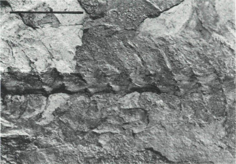
Abb. 7: Sigillariostrobus sp.
