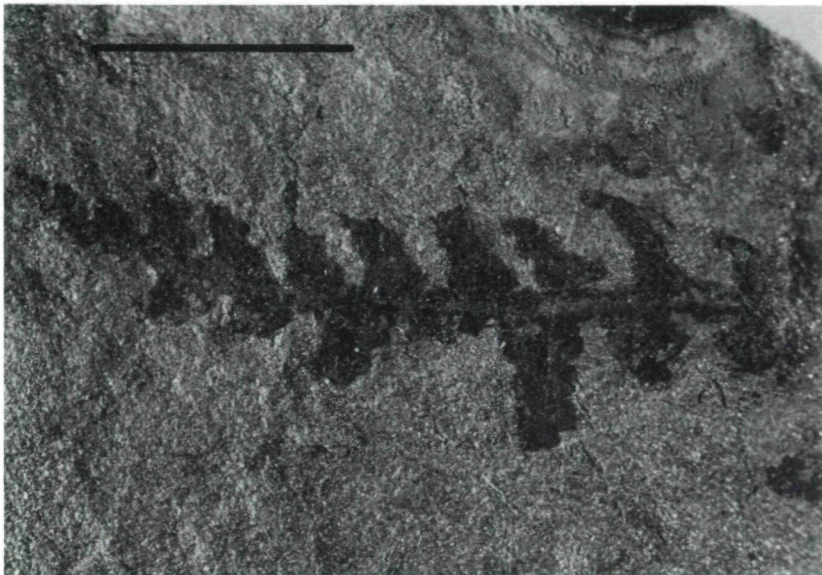
Abb. 35: Sphenopteris sp.
