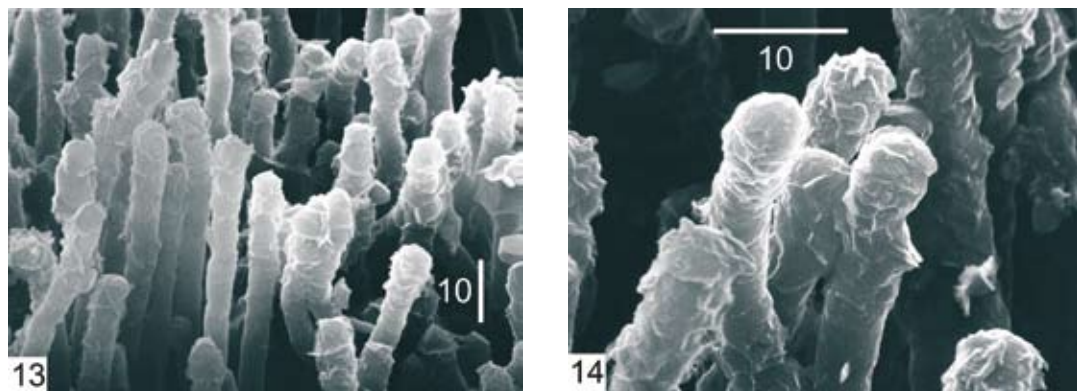
Figs 13-14. Front of Araldite-filled up boring canals showing the calcite crystal structure. Scale bars in µm.
