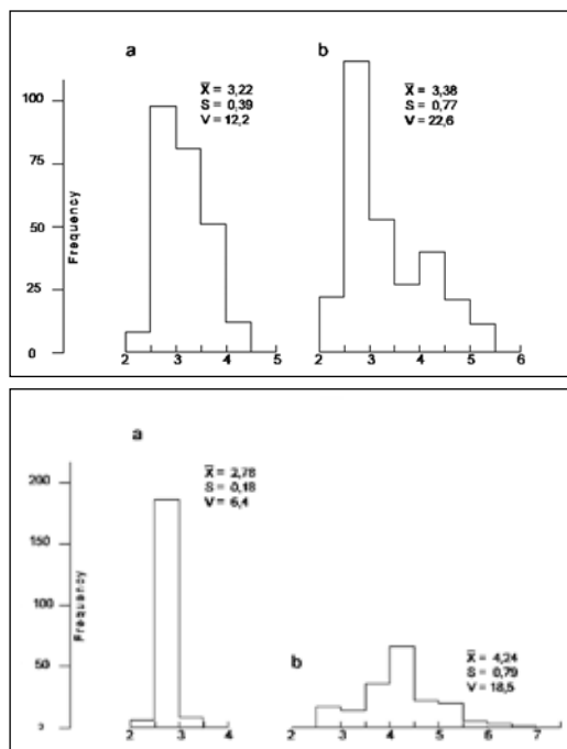
Figs 15, 16. Frequency histograms and statistics for the cell width (a) and cell length (b) of " Phormidium spec. " (fig. 15) and Phormidium corium (fig. 16), established from samples of three different locations, n = 200 each time.
