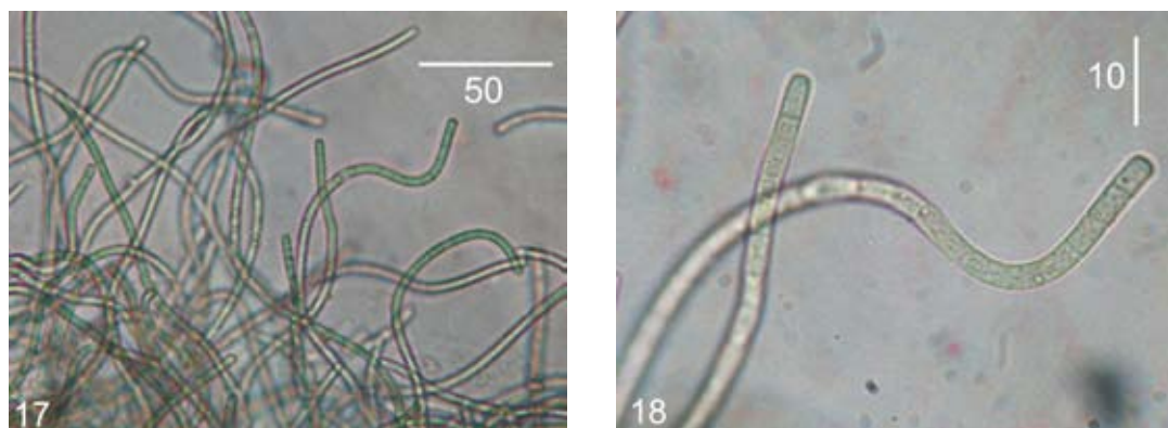
Figs 17, 18. Phormidium corium from a rivulet in the southern Black Forest. Scale bars in µm.
