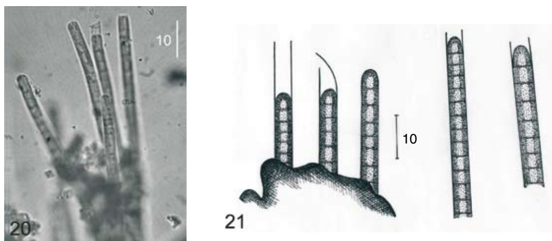
Fig. 20-21. Phormidium ingrediens from river Breg near Hüfingen, south-east edge of the Black Forest. Scale bar in µm.
