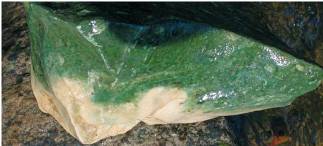
Fig. 1. Limestone with endolithic thallus of Phormidium ingrediens from the river Breg near the town of Hüfingen.
