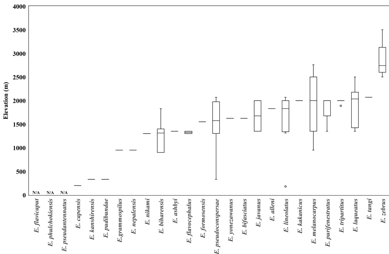
Figure 32. Elevational distribution pattern of the Enicospilus in Nepal.
