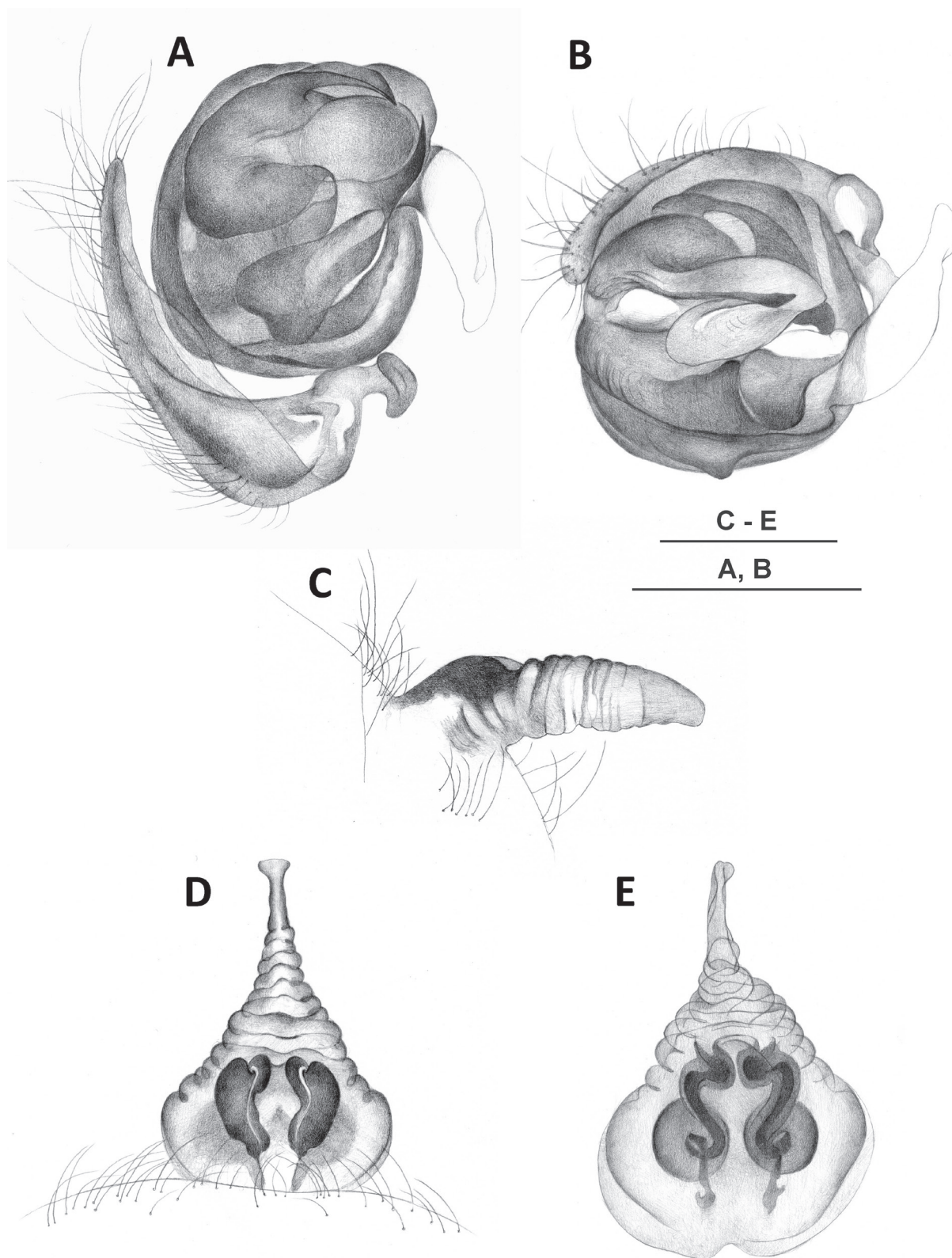
Fig. 3. Eustala orientalis sp. nov. A. ♂ left palp, ventral view. B. ♂ left palp, apical view. C. ♀ scapus, lateral view. D. ♀ epigyne scapus, ventral view. E. ♀, spermathecae. Scale lines = 0.5 mm.
