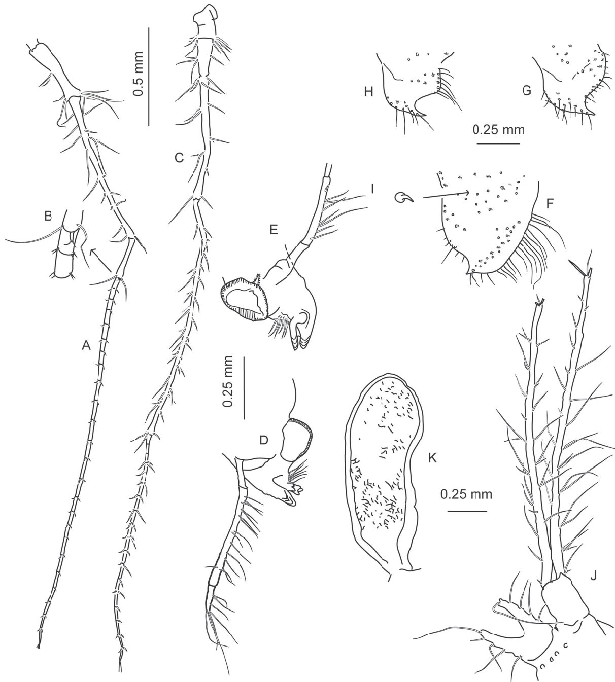
Fig. 9. Lepechinella norvegica sp. nov., allotype, ♀. A. A1. B. Accessory flagellum of A1. C. Female A2. D–E. Right and left mandible. F. Right Ep1. G. Left Ep2. H. Left Ep3. I. Spine on Ep 1. J. Telson and left U3. K. Gill of P3.
