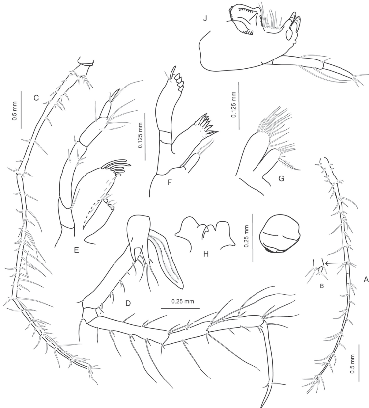
Fig. 18. Lepe subchela christinae gen. et sp. nov., holotype, immature. A–B. A1 with accessory flagellum. C. A2. D. Right P3 with gill. E. Left Mxp. F. Left Mx1. G. Left Mx2. H. Lower lip. I. Upper lip. J. Right mandible.
