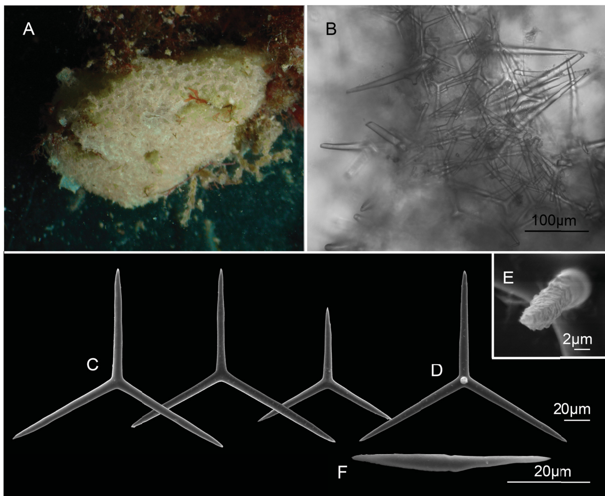
Fig. 2. Asclatis reticulum (PMR 13739 = UFRJPOR 6870). A. Specimen in situ . B. Section showing the perpendicular arrangement of diactines. C. Regular triactines. D. Regular tetractine. E. Apical actine of a tetractine covered with short spines. F. Diactine.
