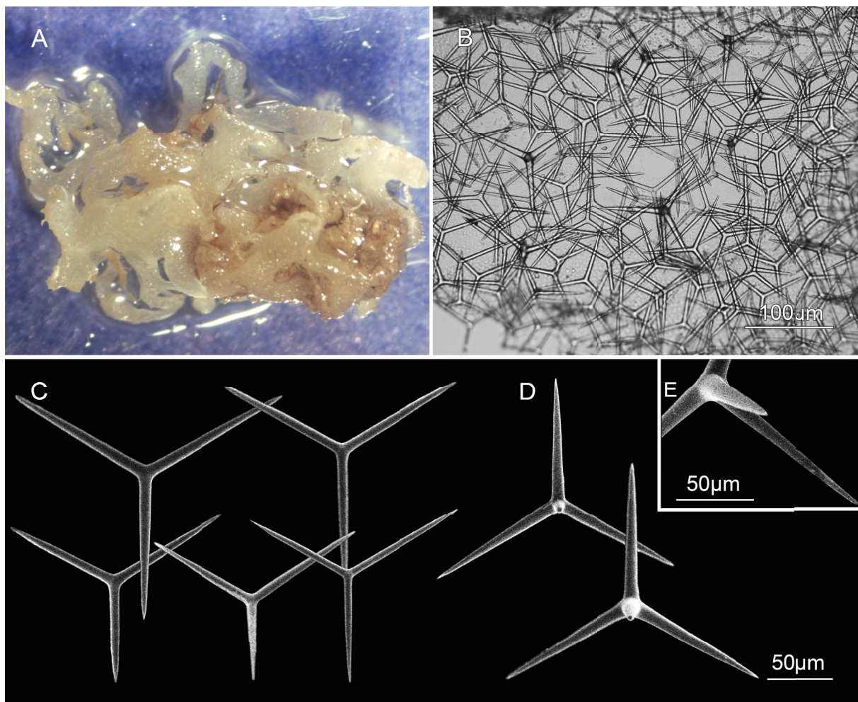
Fig. 3. Ascandra spalatensis sp. nov., holotype (PMR 17806 = UFRJPOR 7540). A. Specimen in ethanol. B. Tangential section. C. Triactines. D. Tetractines. E. Apical actine of a tetractine.
