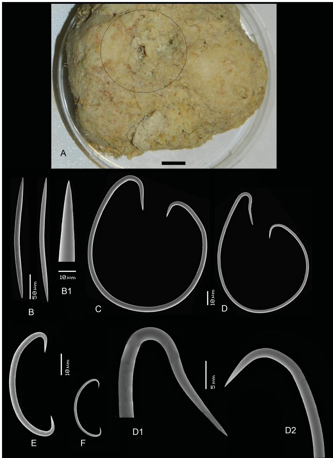
Fig. 10. Haliclona (Flagellia) amirantensis subgen. et sp. nov., holotype (ZMA Por. 12409), from Desnoeufs Island, Amirantes, Seychelles. A. Habitus (encircled) encrusting a large Topsentia specimen (scale bar = 1 cm). B–F. SEM images of the spicules. B. Oxeas. B 1 . Detail of one of the apices. C–D. Flagellosigmas. D 1 . Detail of long ending of flagellosigma. D 2 . Detail of short ending of flagellosigma. E. Large sigma category (I). F. Small sigma category (I).
