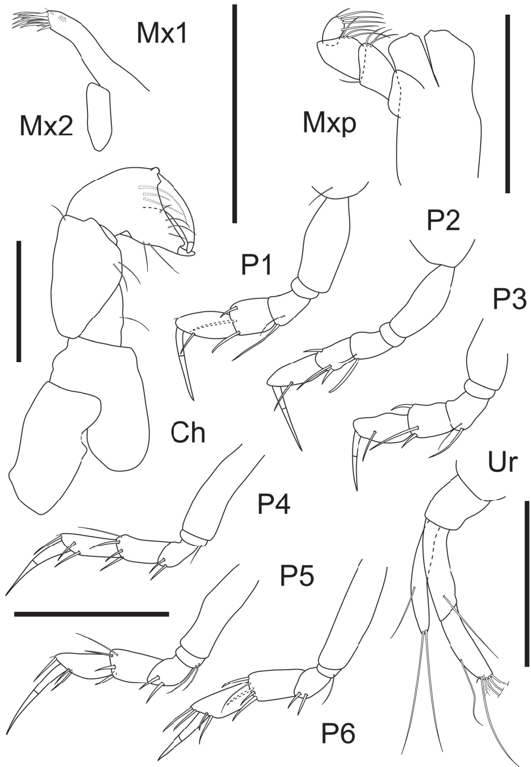
Fig. 3. Filitanaia elongatus sp. nov., holotype, ♀ (MNRJ 24443), length 1.9 mm. Abbreviations: Mx1 = maxillule; Mx2 = maxilla; Mxp = maxilliped; Ch = cheliped; P1 = pereopod 1; P2 = pereopod 2; P3 = pereopod 3; P4 = pereopod 4; P5 = pereopod 5; P6 = pereopod 6; Ur = uropod. Scale bars = 0.1 mm.
