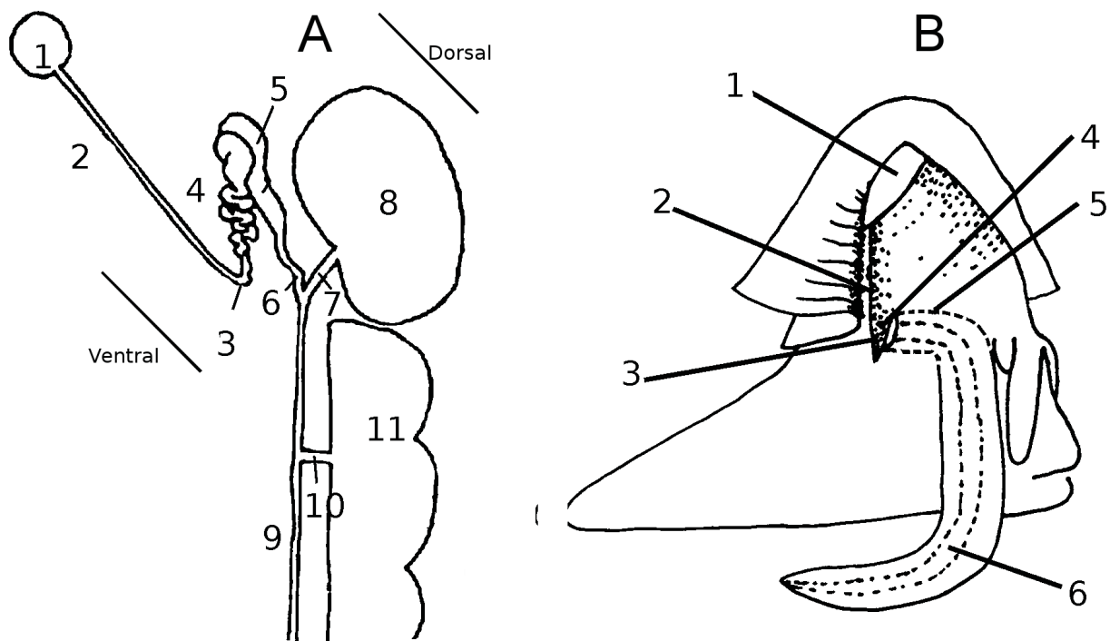
Fig. 3. Genitals of Cochlostoma Jan, 1830. A. Female genitals. 1 = ovary; 2 = visceral oviduct; 3 = proximal loop; 4 = loops of the visceral oviduct; 5 = seminal receptacle; 6 = distal oviduct; 7 = pedunculus of the bursa copulatrix; 8 = bursa copulatrix; 9 = copulatory duct; 10 = channel of the uterine gland; 11 = uterine gland. B. Male genitals. 1 = anus; 2 = groove fold; 3 = sperm pocket; 4 = penial funnel; 5 = body spermiduct; 6 = penis with the penial spermiduct.
