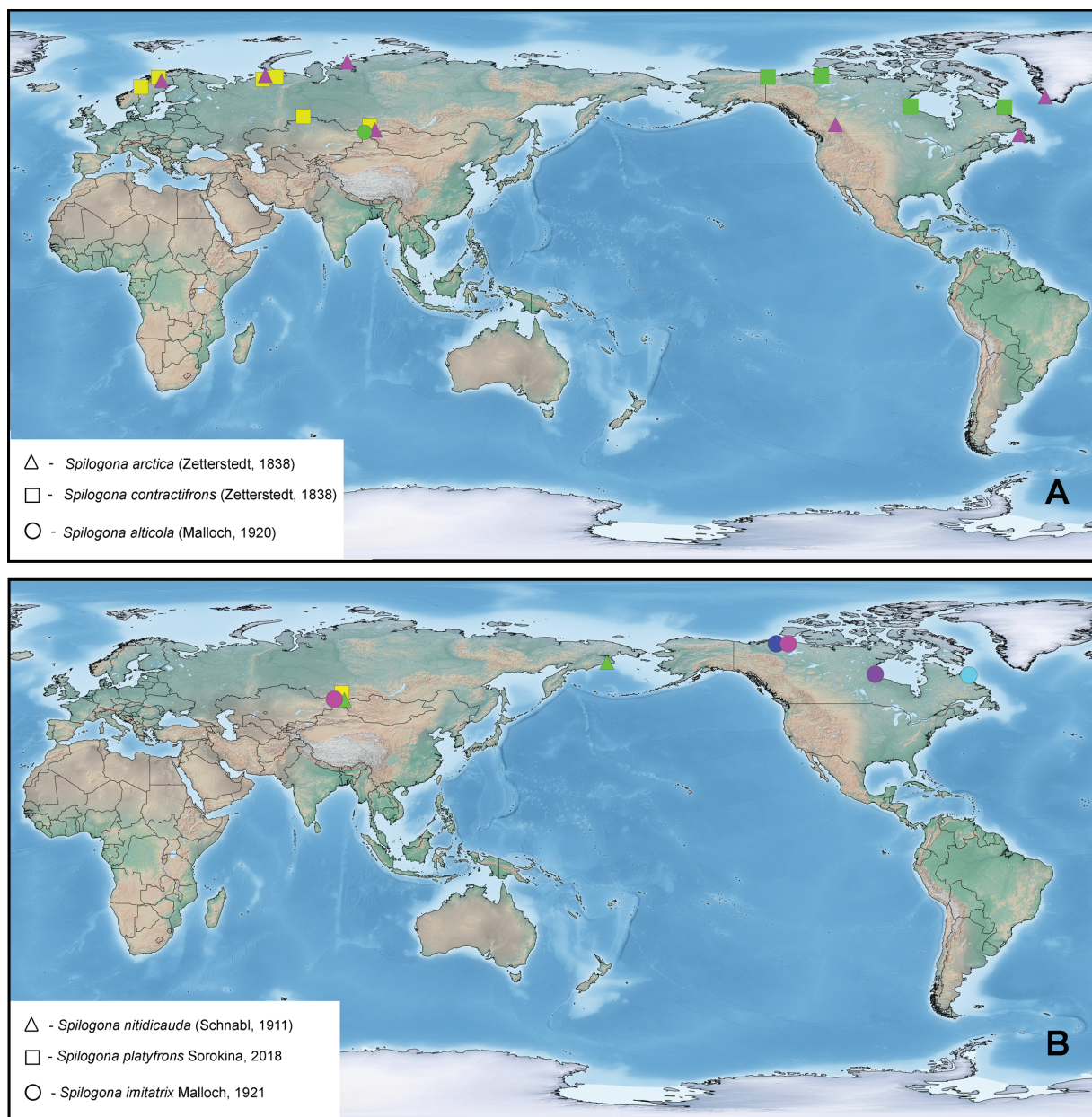
Fig. 6. Localities of the species of Spilogona Schnabl, 1911 used in the DNA analysis. Symbols denote the species, whilst the colour shows the same DNA sequences. A. ' S. contractifrons species-group'. B. ' S. nitidicauda species-group'.
