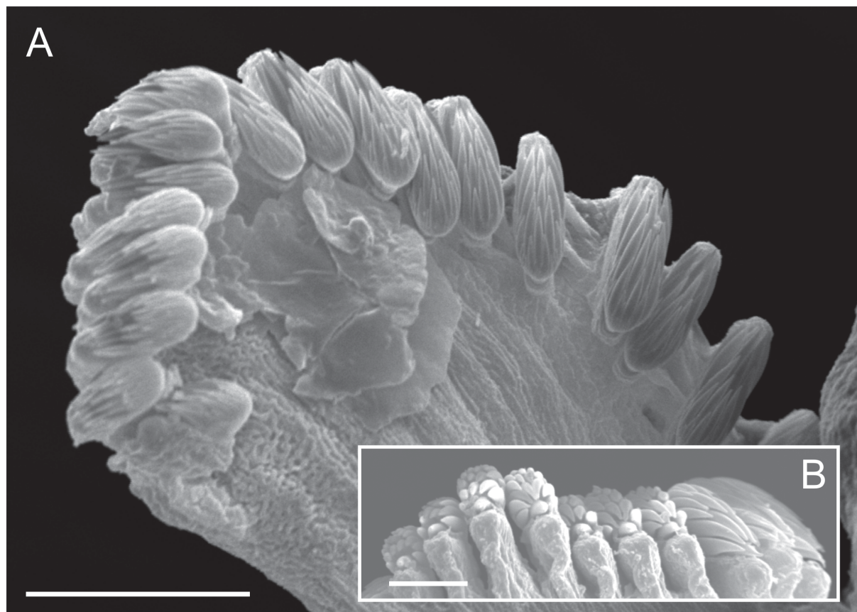
Fig. 6. Ampharete oculicirrata sp. nov., paratype MNCN 16.01/18482_spec. 3. A. Abdominal unciniger 7, posterior view. B. Detail of abdominal uncini, frontal and lateral view. Scale bars: A=150 µm; B = 5 µm.
