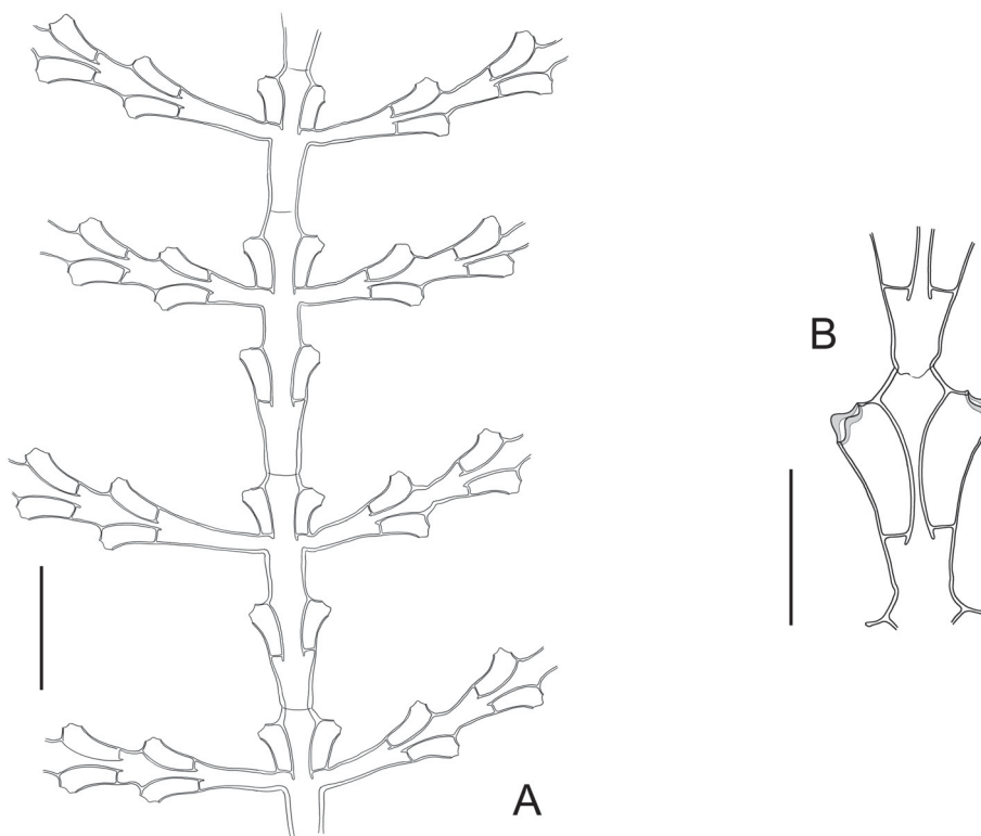
Fig. 11. Dynamena opposita Galea, sp. nov. A–B. Distal part of colony showing branching pattern (A), cladial internode with pair of hydrothecae (B). Scale bars: A = 1 mm; B = 500 µm.
