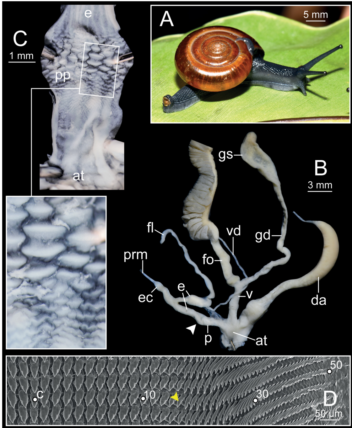
Fig. 5. Sarika khmeriana Pholyotha & Panha sp. nov., paratype (CUMZ 7905). A. Living snail. B. Benel view of genital system. C. Internal structure of penis. D. Representative SEM image of the radula. Central tooth indicated by 'C'; yellow arrow heads indicate lateral teeth with the transition to marginal teeth; white arrow heads indicate the end of penis.
