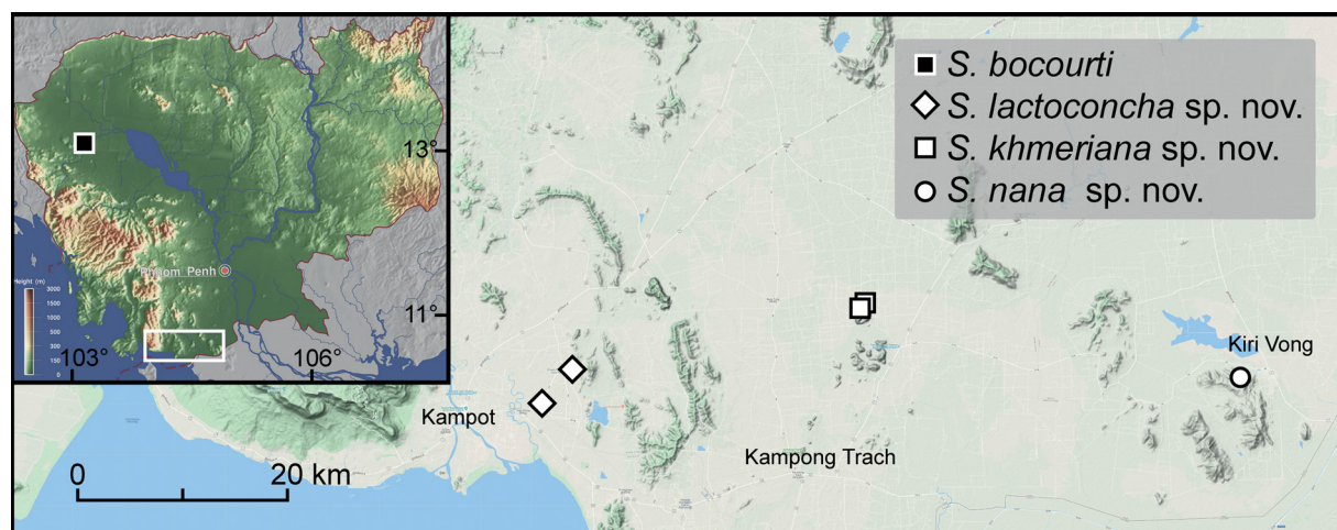
Fig. 1. Geographic distribution of Sarika spp. in Cambodia based on new specimens examined herein. (modified from GinkgoMaps-project http://www.ginkgomaps.com ).
