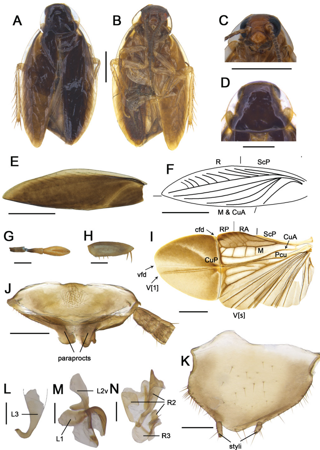
Fig. 7. Anaplecta cruciata Deng & Che sp. nov., holotype, ♂ (SWU). A. Habitus, dorsal view. B. Habitus, ventral view. C. Head, ventral view. D. Pronotum, dorsal view. E. Tegmina. F. Tegnina vein. G. Maxillary palp. H. Front femur, ventral view. I. Wings. J. Supra-anal plate, dorsal view. K. Subgenital plate, ventral view. L. Hook, ventral view. M. Left phallomere, ventral view. N. Right phallomere, ventral view. Scale bars: A–C=1 mm; D–F, I–K=0.5 mm; G–H=0.2 mm; L–N=0.25 mm.
