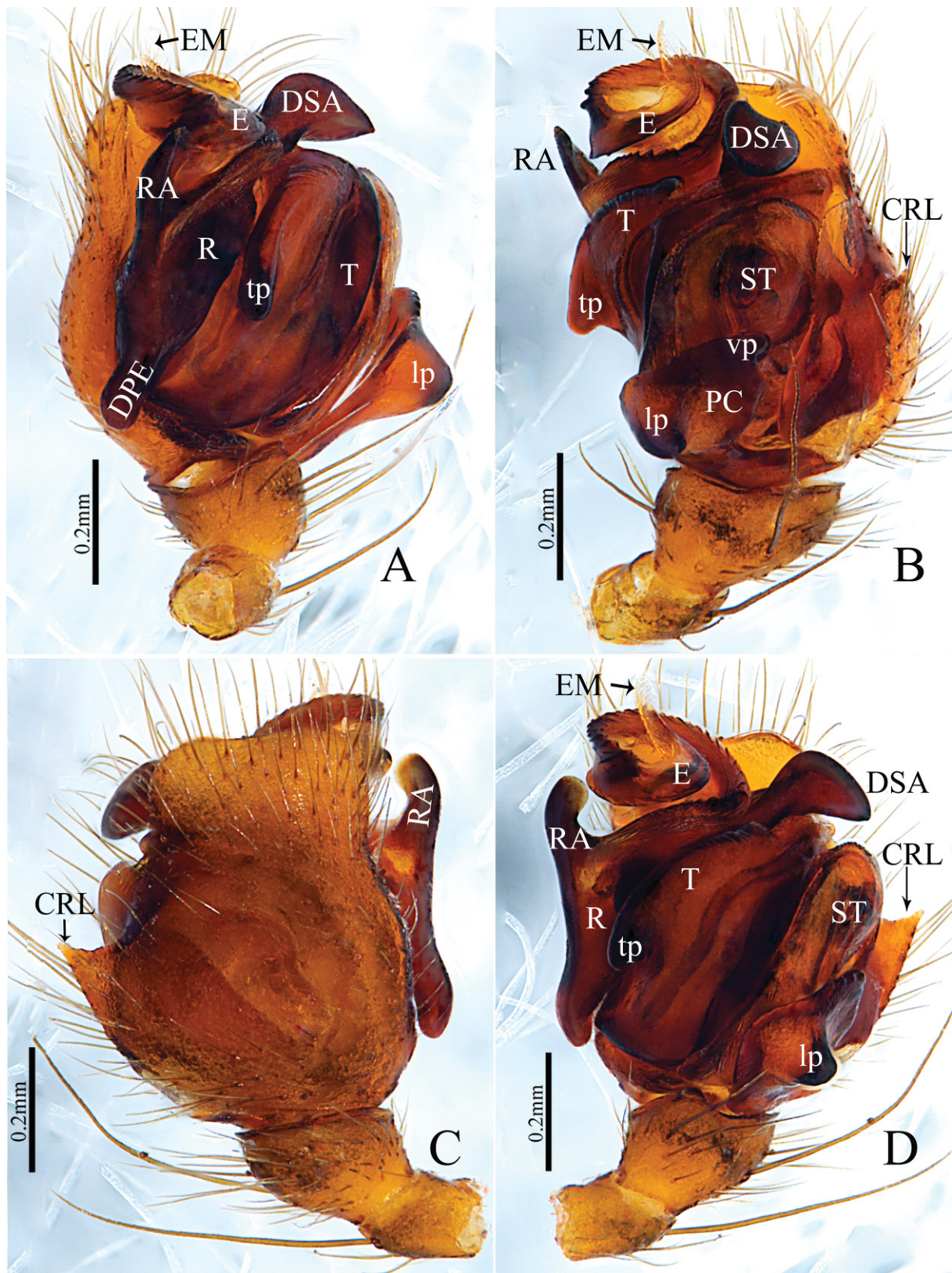
Fig. 15. Acroterius circinatus gen. et sp. nov., ♂, holotype (HNU-CGY137), palp. A. Prolateral view. B. Retrolateral view. C. Dorsal view. D. Ventral view.
