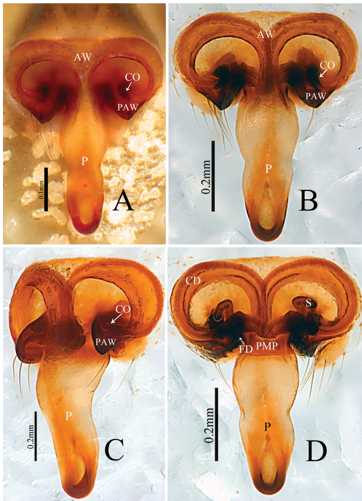
Fig. 32. Acroterius longimultus gen. et sp. nov., ♀, paratype (HNU-20040501–02). A–B. Epigyne, ventral view. C. Epigyne, lateral view. D. Vulva, dorsal view.
