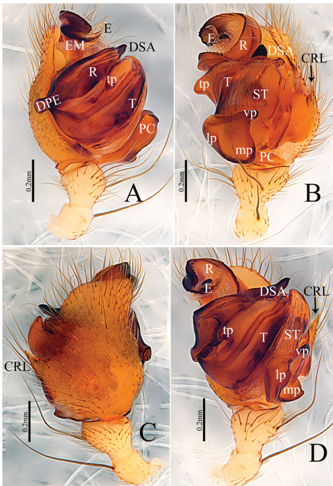
Fig. 1. Acroterius absentus gen. et sp. nov., ♂, holotype (HNU-Tang031027), palp. A. Prolateral view. B. Retrolateral view. C. Dorsal view. D. Ventral view.
