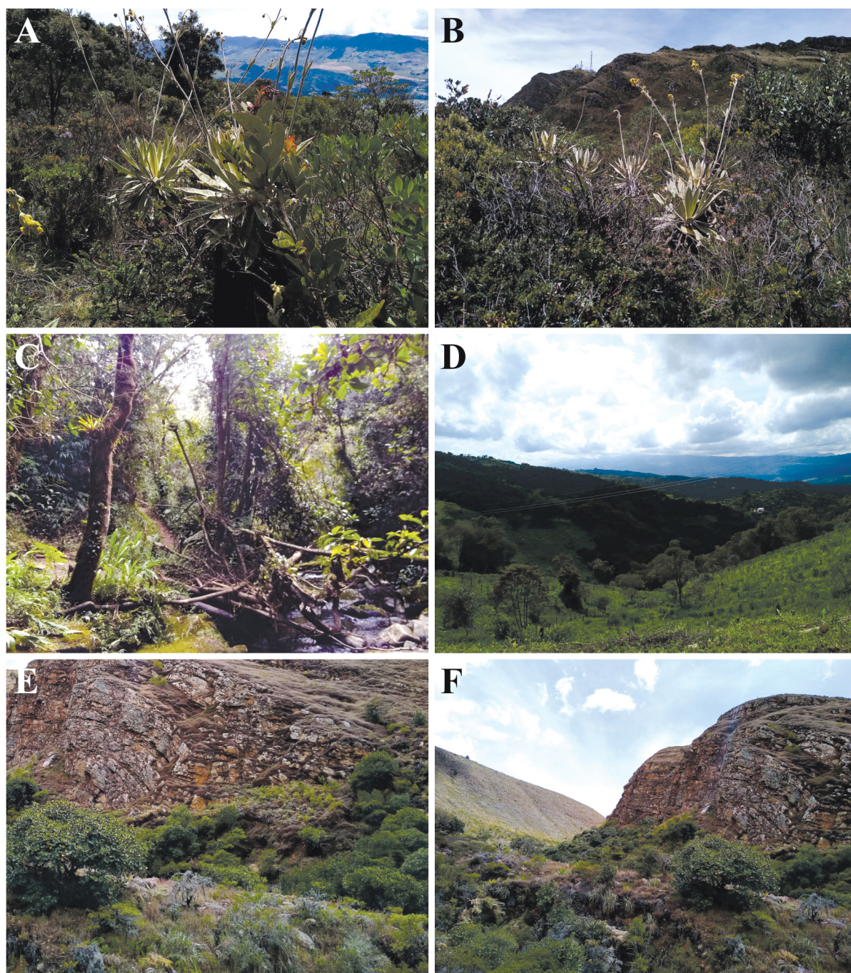
Fig. 8. Habitats of Colombian species of Medionops Sánchez-Ruiz & Brescovit, 2017. A–B. Type locality of M. blades Sánchez-Ruiz & Brescovit, 2017, Páramo de Monserrate, Cundimarca department, Colombia. C–D. Type locality of M. carolinae sp. nov., Sutamarchán, Boyacá department, Colombia. E–F. Habitat of female paratype (IAvH-I 3771) of M. carolinae sp. nov., Sector Carrizal, Santuario de Flora y Fauna Iguaque, Boyacá department, Colombia.
