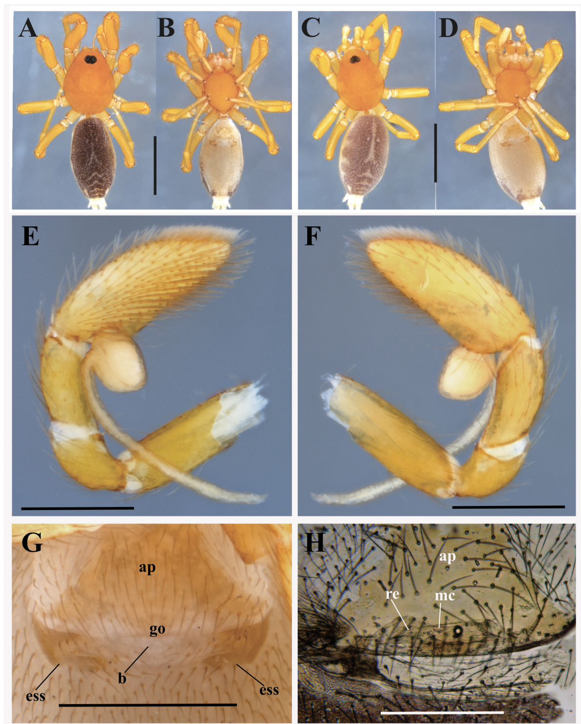
Fig. 4. Medionops luiscarloshi sp. nov. A–B, E–F. Holotype, ♂ (IAvH-I 3361). C–D, G–H. Paratype, ♀ (IAvH-I 3772). A. Habitus, dorsal view. B. Habitus, ventral view. C. Habitus, dorsal view. D. Habitus, ventral view. E. Left palp, retrolateral view. F. Left palp, prolateral view. G. External genitalia, ventral view. H. Internal genitalia, dorsal view. Scale bars: A–D = 1.5 mm; E–F = 0.7 mm; G = 0.5 mm; H = 0.2 mm. Abbreviations: p = anterior plate; b = area below genital opening; ess = external sclerotization around spiracles; go = genital opening; re = receptaculum; mc = median concavity.
