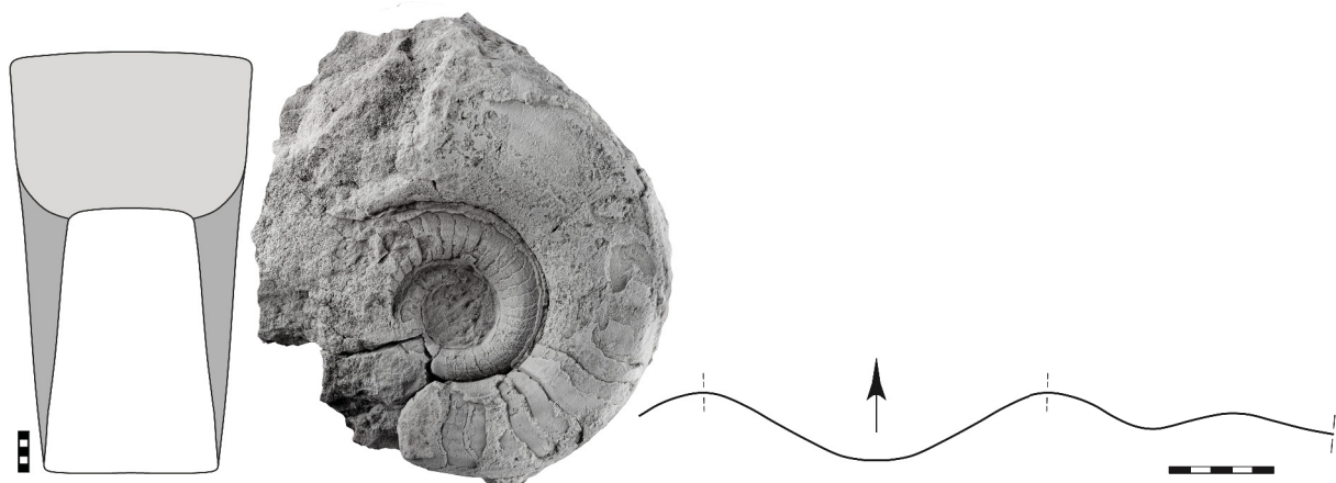
Fig. 9. Rinecerases rectangulatum sp. nov., dorsal view reconstruction, lateral view and suture line (at 36 mm dm, 21 mm ww, 14 mm wh) of holotype MB.C.30382. Scale bar units = 1 mm.
