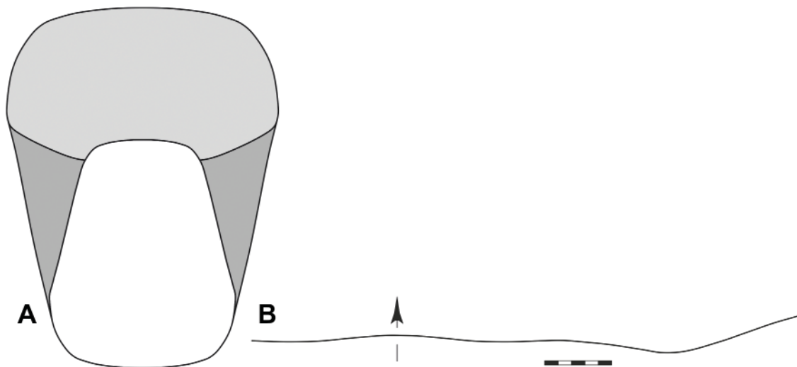
Fig. 13. Planetoceras destrictum sp. nov., holotype MB.C.30385. A. Dorsal view reconstruction. B. Suture line at 52 mm dm, 42 mm ww, 22 mm wh. Scale bar units = 1 mm.
