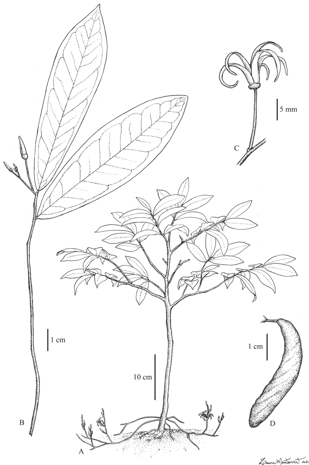
Fig. 2. Morphological characters of Hornschuchia bryotrophe Nees. A. Habit, showing the cauliflorous inflorescence emerging from the base of the trunk with inflorescence branches highly ramified (J.C. Lopes III, SPF). B. Inflorescence branch with floral buds (J.R. Pirani 3074, SPF). C. Flower (L.F.S. Magnago 1646, SPF). D. Monocarp (C. Rocchini 7, SPF). Drawing by Laura Montserrat.
