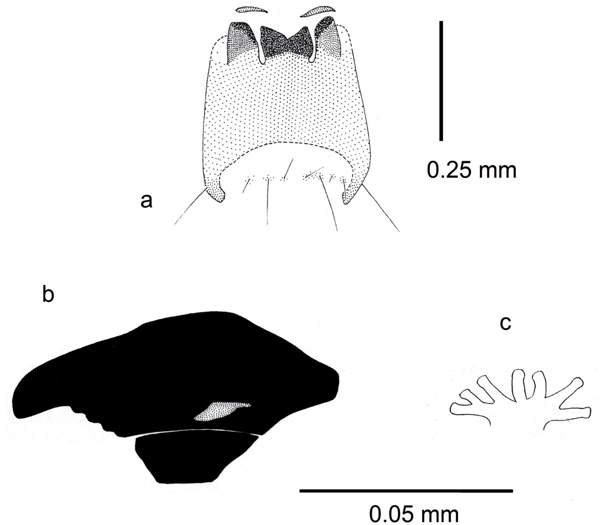
Fig. 3. a. Atherigona subnigripes (Karsch, 1888), holotype, ♀ (MNB), eighth tergite, dorsal. b–c. Atherigona varia (Meigen, 1826). b. Larval mandibular sclerite, lateral. c. Anterior spiracle of puparium.
