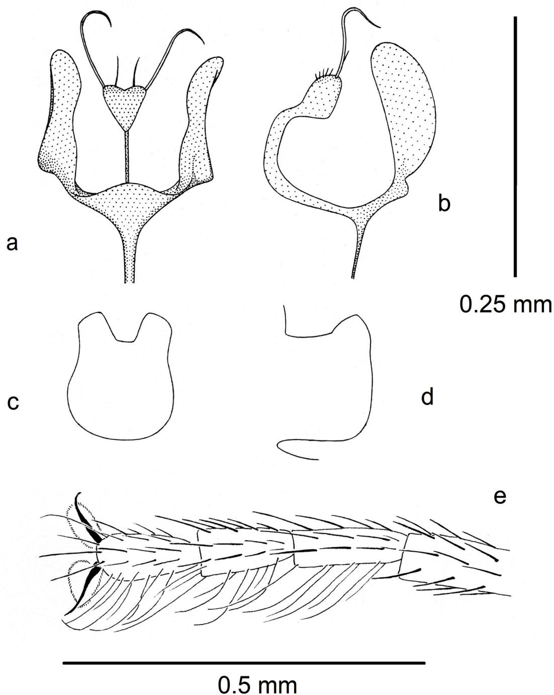
Fig. 4. Atherigona zongoi sp. nov., holotype, ♂ (NMWC). a. Trifoliate process, ventral. b. Same, lateral. c. Hypopygial prominence, posterior. d. Same, lateral. e. Fore tarsus.
