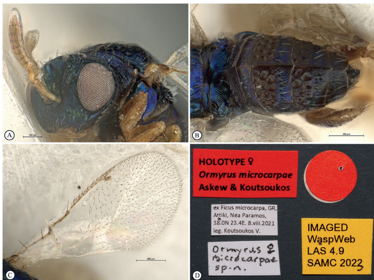
Fig. 2. Ormyrus microcarpae Askew & Koutsoukos sp. nov., holotype, ♀ (NHMUK). A. Head and mesosoma, antero-lateral view. B. Metasoma, dorsal view. C. Fore wing. D. Labels.
