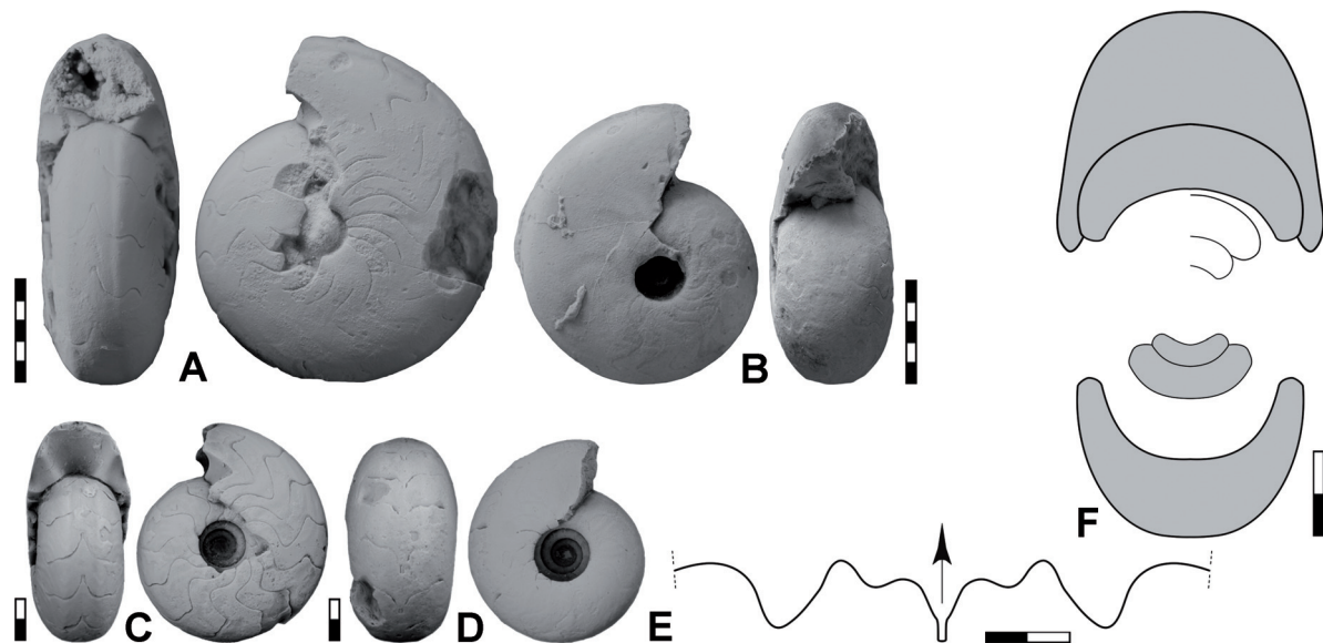
Fig. 4. Maenioceras afroterebatum sp. nov. A. Holotype MB.C.31947.1 from Oued Mzerreb-W, bed 6. B. Paratype MB.C.31948.1 from Oufrane-W, bed 3. C. Paratype MB.C.31947.2 from Oued Mzerreb-W, bed 6. D. Paratype MB.C.31948.2 from Oufrane-W, bed 3. E. Paratype MB.C.31947.2 from Oued Mzerreb-W, bed 6; suture line at dm = 10.0 mm. F. Paratype MB.C.31947.3 from Oued Mzerreb-W, bed 6; cross section. Scale bar units = 1 mm.
