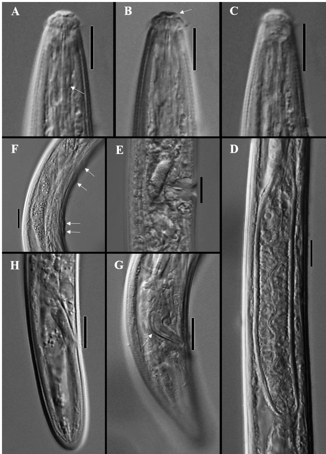
Fig. 3. Dorylaimellus discocephalus Siddiqi, 1964 (LM photographs). A. Anterior region, arrow indicating basal flanges. B. Arrow indicating perioral disc. C. Anterior end showing amphid. D. Expanded part of pharynx. E. Vulva. F. Arrows indicating ventromedian supplements. G. Male posterior end, arrow indicating spicule. H. Female posterior end. Scale bars: A–H = 10 \mu m.
