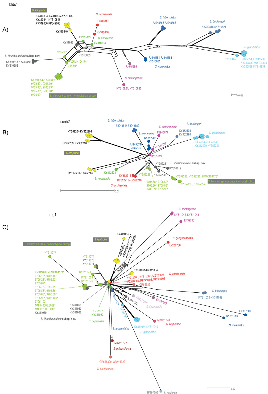
Fig. 3. Neighbor-Net networks (Bryant & Moulton 2004) of the nuclear genes retrieved in Scutigera Theobald, 1868. A. Beta-fibrinogen gene, intron 7. B. Cyclin B2 gene, intron 3. C. Rag1 gene.
