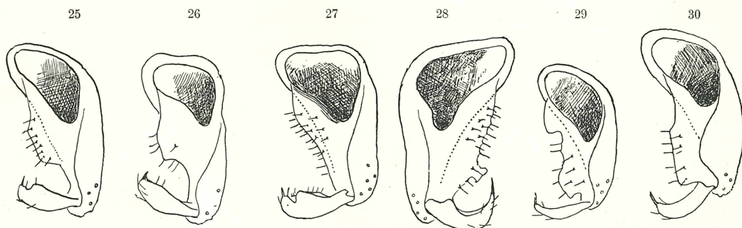
Textfigg. 25—30. Hypopygien (Hälften) von Thienemanniella flaviscutellata Tok. (25), Th. nipponica Tok. (26), Corynoneura cuspid Tok. (27), C. longipennis Tok. (28), C. tenuistyla Tok. (29) und C. yoshimurai Tok. (30) (nach Tokunaga).
