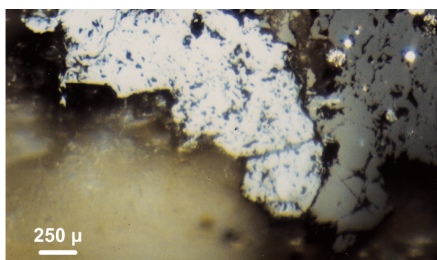
FIG. 12: Ore microscopy showing paragenesis of the uranium/copper mineralisation. A: Covellite (blue) is replaced by tennantite (cream). (Brantental, oil, polarized light). B: Uraninite (white) and pyrite (grey) in coal (black) (Moelten, oil, polarized light).
