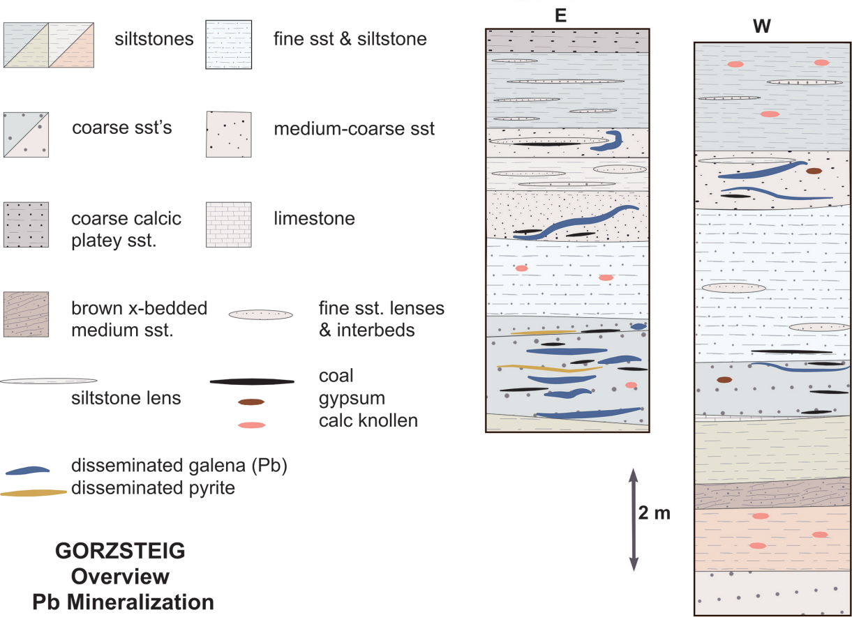
FIG 14: Profiles at the locality Gorzsteig show the interdependence of galena and sphalerite mineralisation and lithology.
