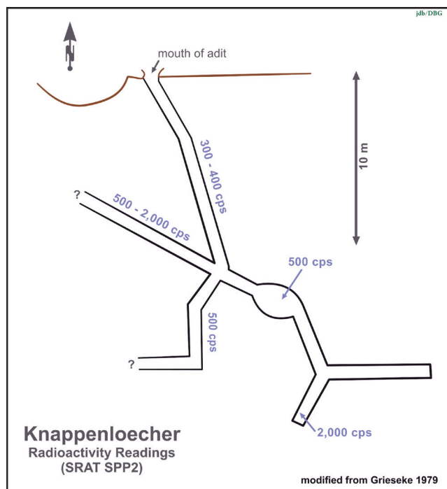
FIG. 8: Plan of the adits of Knappenloch and intensity of gamma-radiation shown in counts per second (cps), measured in the various sectors of the adits (modified from Griesseke, 1979).
