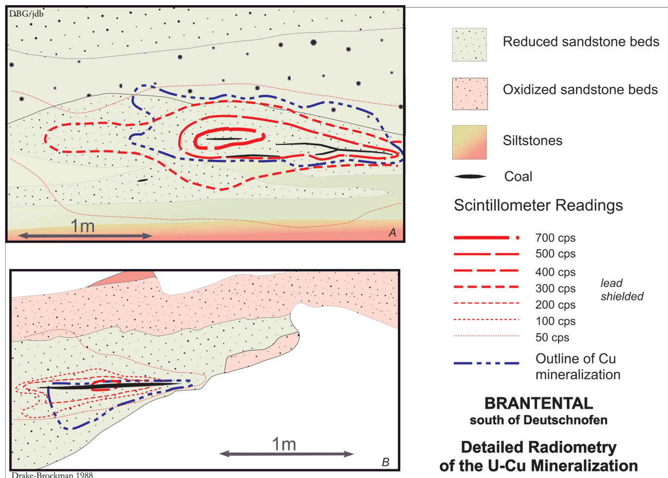
FIG. 9: Examples of Cu and U mineralisation in the upper Brantental. (A) shows how isoradiants (lines of equal radioactivity) are extended in the direction of bedding of the mineralized coal seam. (B) demonstrates how the bedding is cut obliquely by the reduction front (modified from Drake-Brockman, 1988).
