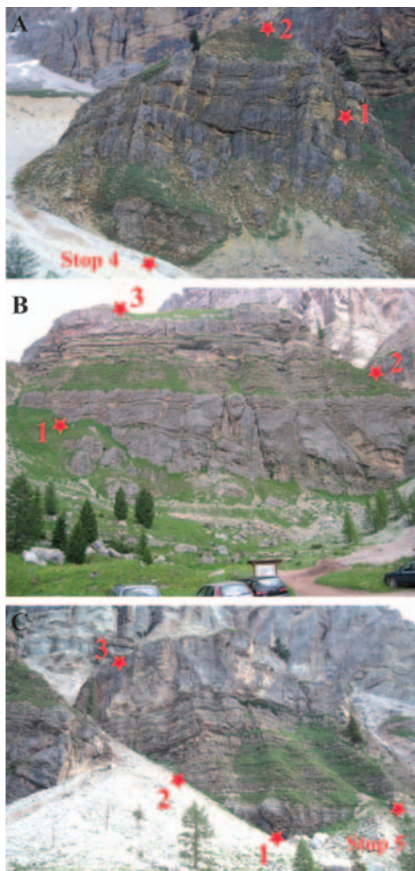
Fig. 13: Views of the Heiligkreuz Fm. from Rifugio Dibona. 1: Borca member, dolomitized prograding shoal barrier; 2: Dibona Sandstones member; 3: Lagazuoi member. A) The clineostratified shoal barrier is visible in the western tower, as well as the underlying part of the Borca member. B) clineoforms are most evident in the wall in front of the hut. Pay attention to some fallen blocks of layered dolostone, which tilting mimics the dip of clineoforms. C) Deep incisions allow bed-by-bed measurement of the whole Heiligkreuz and Travenanzes formations.
