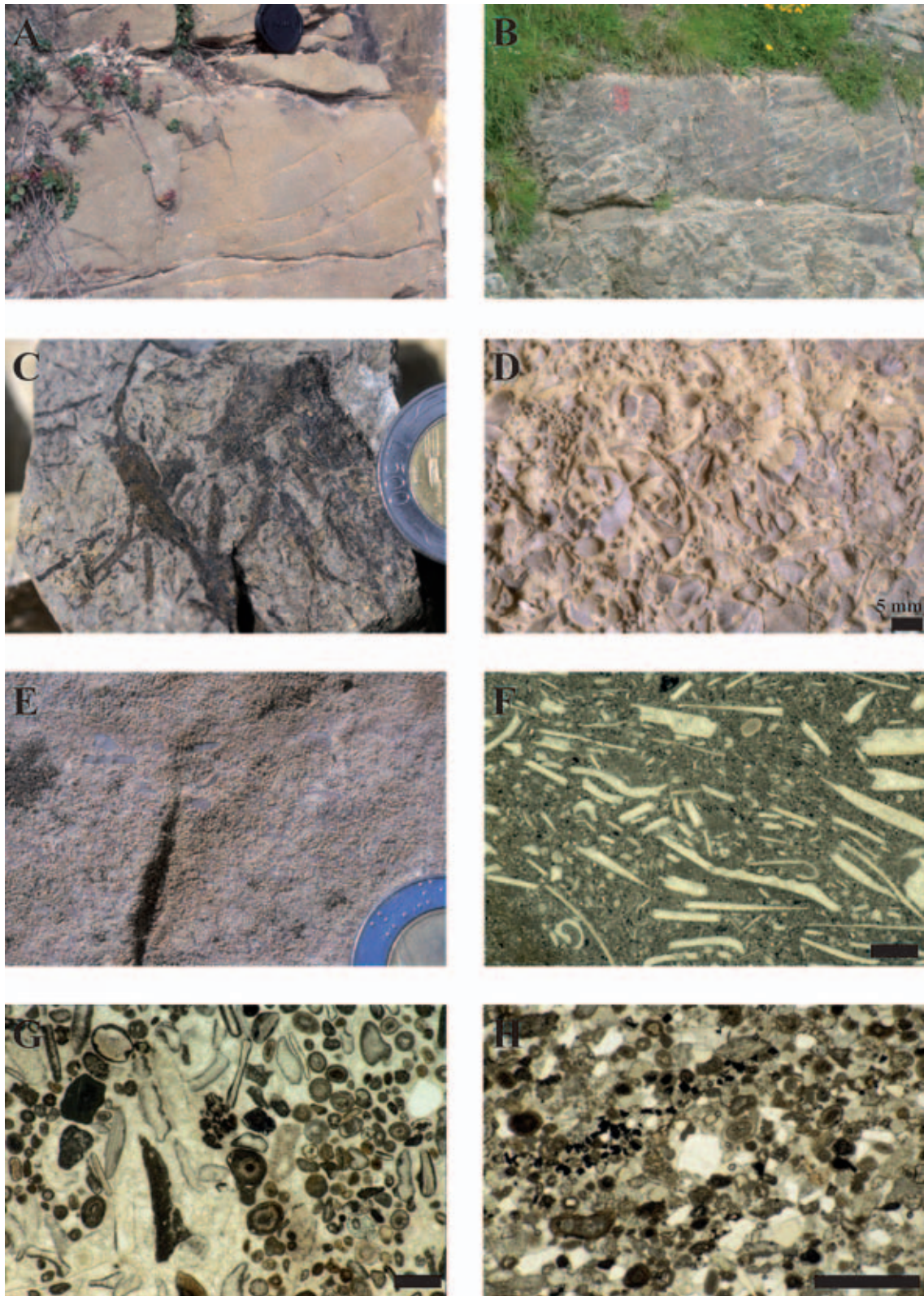
Fig. 18: Facies and microfacies of the upper Borca and Dibona Sandstones members. Scale bars for microfacies = 1mm, coin = 16 mm. A) dm-scale tangential cross-bedding in oolitic-bioclastic calcarenites of facies association E; B) planar cross-bedding; C) roots in silty marls of facies association E; D) oolitic-bioclastic grainstone (facies association E), with bivalves, gastropods, ostracods, brachiopods, echinoderms; E) flat pebbles in oolitic grainstone (facies association E); F) packstone with fractured bivalve shells (facies association E); G) oolitic-bioclastic grainstone (cf. D); H) hybrid arenite of facies association E.
