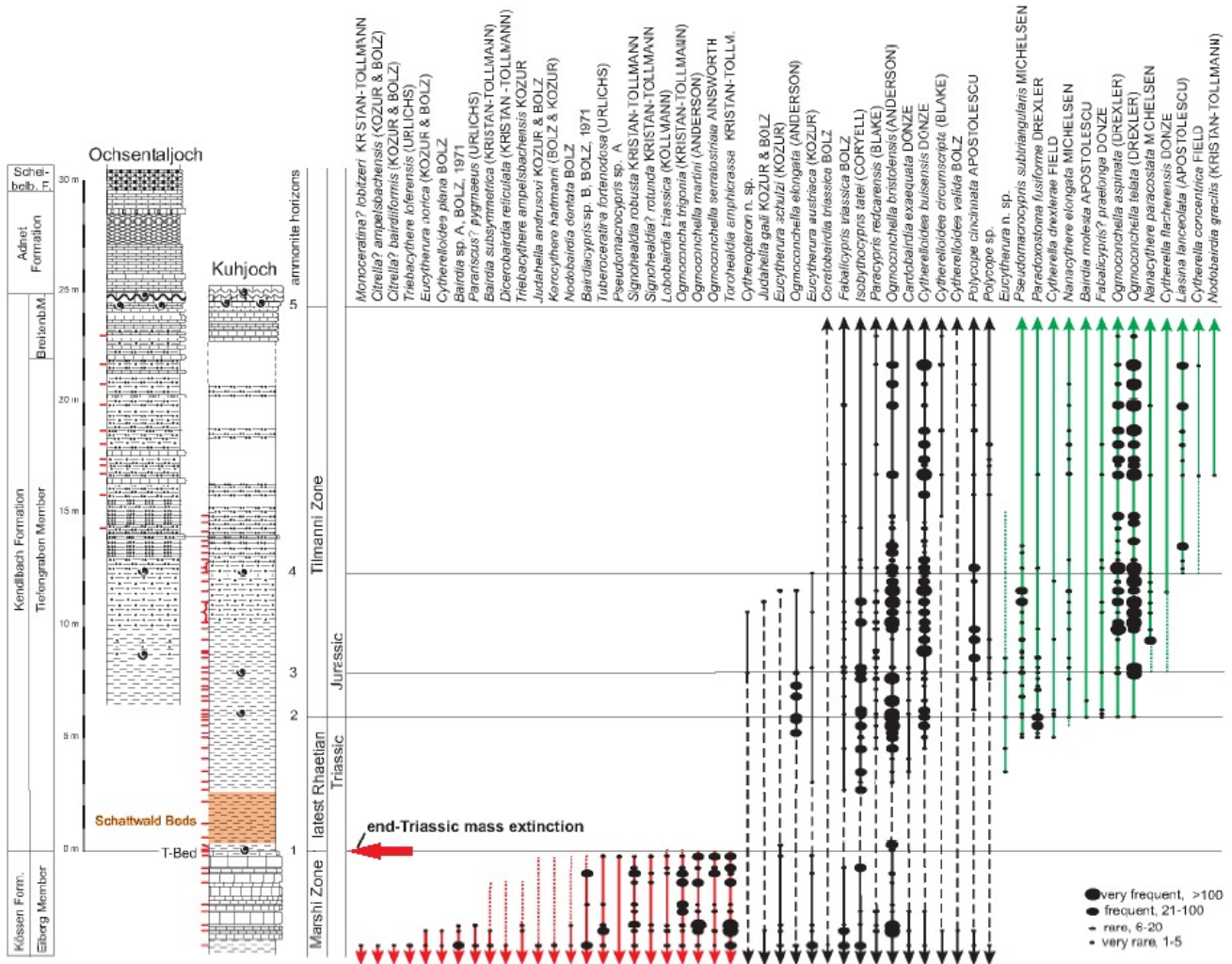
Fig. 14: Range of ostracod taxa at the Kuhjoch and Ochsentaljoch sections. The numbers 1-5 represent ammonite levels: 1= Choristoceras marshi , 2= Psiloceras spelaie tirolicum , 3= Psiloceras ex.gr. P. cf. tillmanni , 4= Psiloceras cf. pacificum (modified after Hillebrandt et al., 2013).
