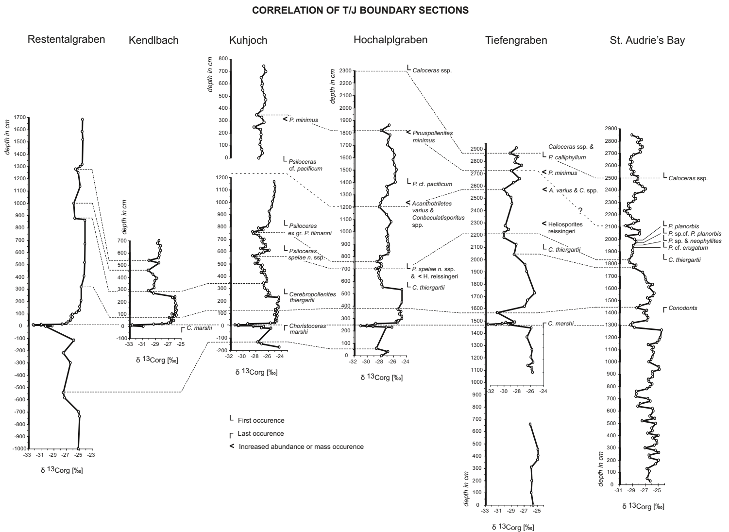
Fig. 17: Stratigraphic correlation of the Triassic-Jurassic boundary sections from the Northern Calcareous Alps and St. Audrie's Bay based on high resolution organic C-isotope records and biostratigraphic markers (modified after Ruhl et al. 2009).
