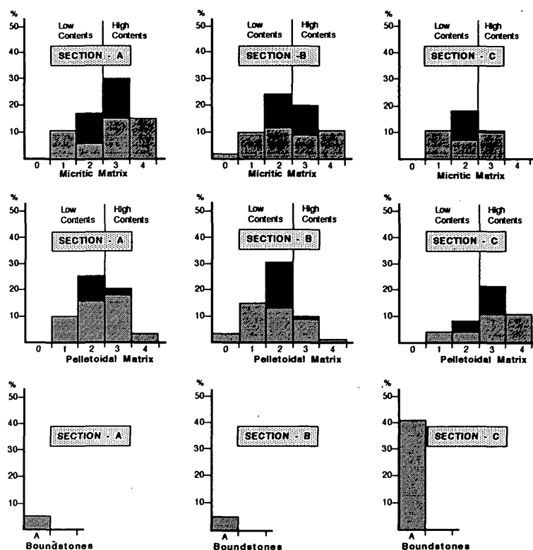
Fig. 5: Frequency of micritic matrix, peloidal matrix and boundstones in the sections A, B and C. The numbers indicate estimated frequencies: 0 = absent, 1 = rare, < 5%, 2 = common, 5-10%, 3 = abundant, 10-20%, 4 = very abundant, > 20%. The histograms are summarized as black bars; 'low' and 'high' contents correspond to rough estimations.
