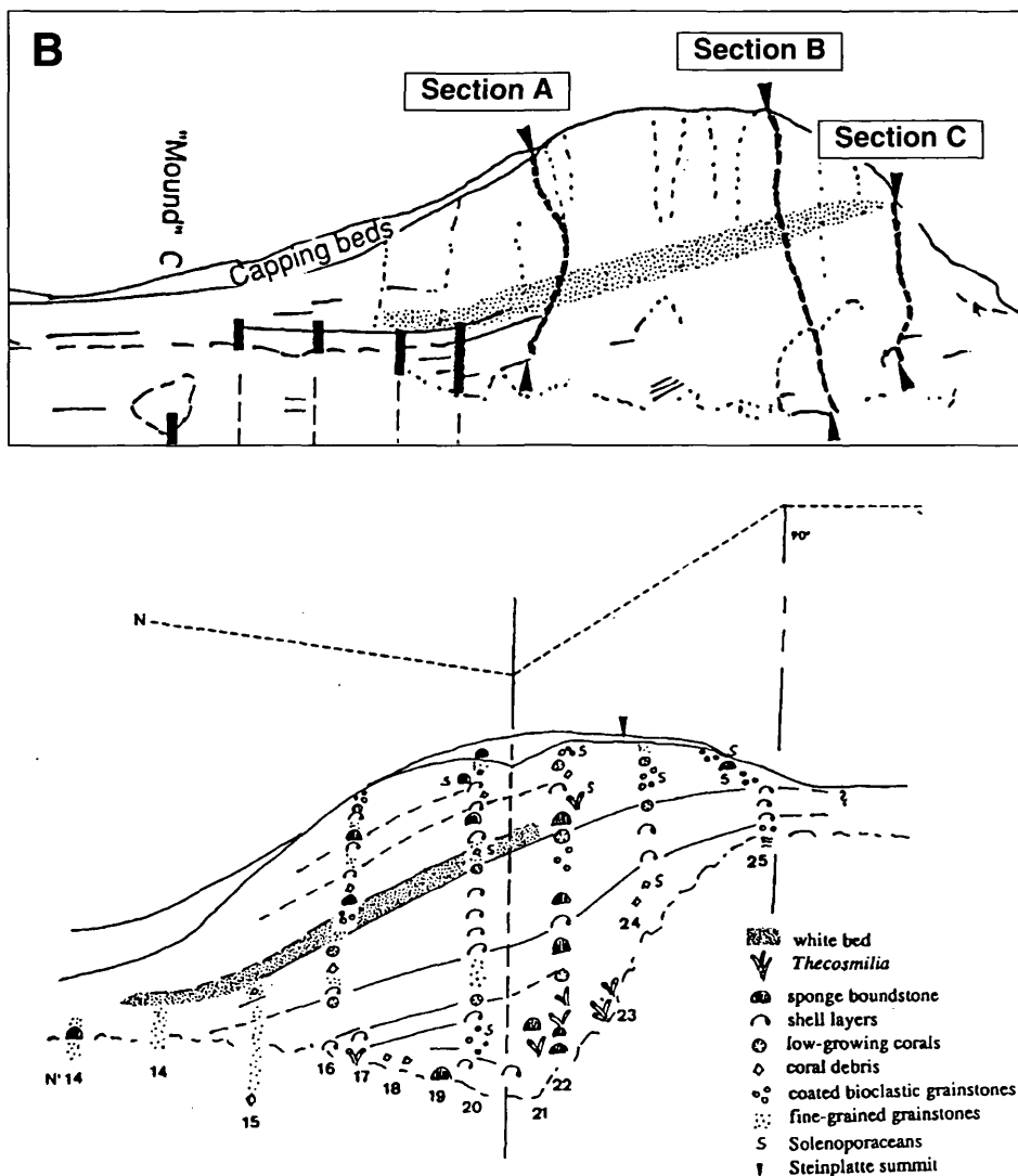
Fig. 3: Distribution of facies criteria within the mound facies. Numbers refer to sampling localities. Lateral and vertical distances are not to scale. The carbonate ramp (right) becomes distally steepened in the vicinity of section D (locality 24) and changes into a distinct slope marked by shell bed III and the 'White Bed'. Note the changes in the thickness of shell bed III (shell symbol; about 25 m in the Wieslochsteig section (locality 25), 8 m in section D, 26 m in section B and 5 m in section A). Boundstones are more common in section C and in the beds overlying the 'White Bed'. Modified from STANTON & FLÜGEL (1989).
