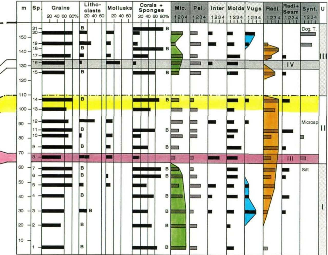
Fig. 4: Distribution of grains, matrix, porosity types and carbonate cements in profiles A, B and C and correlation of the profiles. Legend: Sp. - Sample Mic. - Micritic matrix Pel. - Peloidal matrix Inter - Interparticle porosity Radi - Radial-fibrous cements +Seam - RFC separated by reddish-dusty layers Synt. - Syntaxial overgrowth Microsp. - Microsparitic matrix (recrystallized) Scal. - Scalenohedral calcites U - Unit
