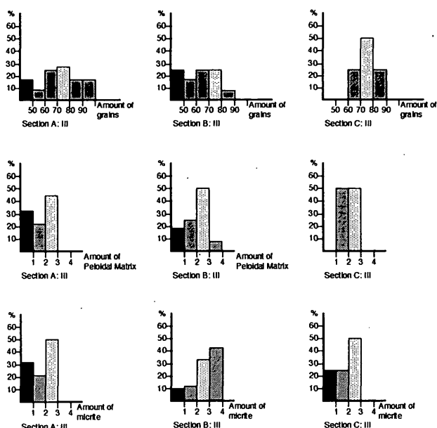
Fig. 8: Frequency of grains and matrix types within rock unit-III in sections A, B and C. For legend see Fig. 5.
