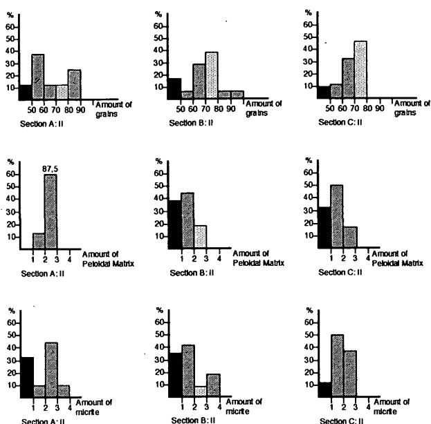
Fig. 7: Frequency of grains and matrix types within rock unit-II in sections A, B and C. For legend see Fig. 5.
