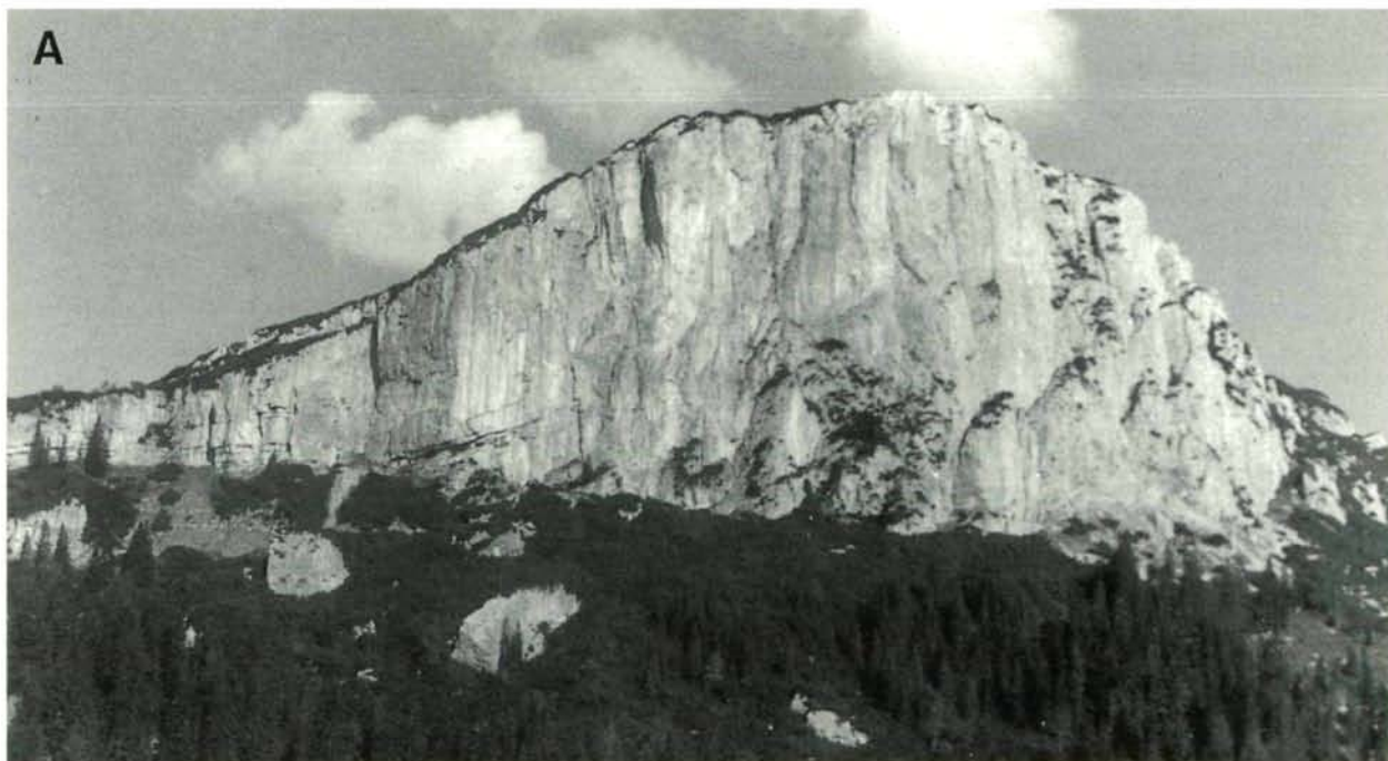
Fig. 2: Study area. A. Western cliff wall of the Steinplatte. The photograph, taken from the Grünwaldkopf, exhibits the bedded and massive Kössen beds grading laterally and vertically into the limestone of the Steinplatte (‘Oberrhätkalk’). Distinct downslope bedding is visible in the transitional area between Oberrhätkalk and flat lying Kössen beds. The cliff comprises the ‘mound facies’ (about 150 m) which is overlain by the onlapping beds of the thin ‘capping facies’ on the flank of the Steinplatte (visible at the top left). The capping facies includes the ‘coral gardens’ on the northern slope of the Steinplatte and the eastern slope of the Plattenkogel. B. Sketch showing the location of the sections studied A (route 5), B (route 12) and C (route 21). The ‘White Bed’ dipping about 20° west is dotted. Modified from STANTON & FLÜGEL (1989).
