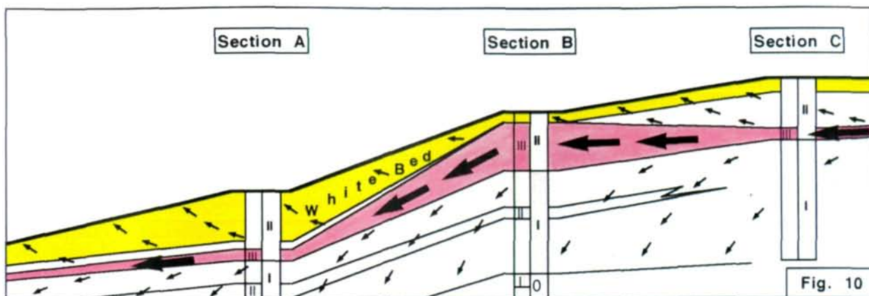
Fig. 10: Sketch of the hydrological system acting subsequent to the deposition of the 'White bed' and influencing the depositional units I and II. An early meteoric influx, using the permeable 'White bed' as conduit caused recrystallization to microspar in the underlying beds and local formation of vugs which were later filled by granular cement. In the 'White bed' primary aragonitic grains are dissolved. Subsequent influx of marine pore waters resulted in the formation of RFC on mollusk shells and boundstone substrates. Arrows indicate pore water flux.
