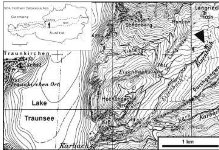
Text-Fig. 1: Geographical setting of the type-locality of Thrysoaporella eisenbachensis n. sp. marked with an asterisk (from ÖK 25, sheet 67 Grünau im Almtal).
