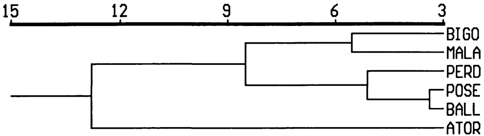
Fig. 3: UPGMA dendrogram based on Mahalanobis distances of grouped samples of male Iberolacerta bonnali (see table 4).
