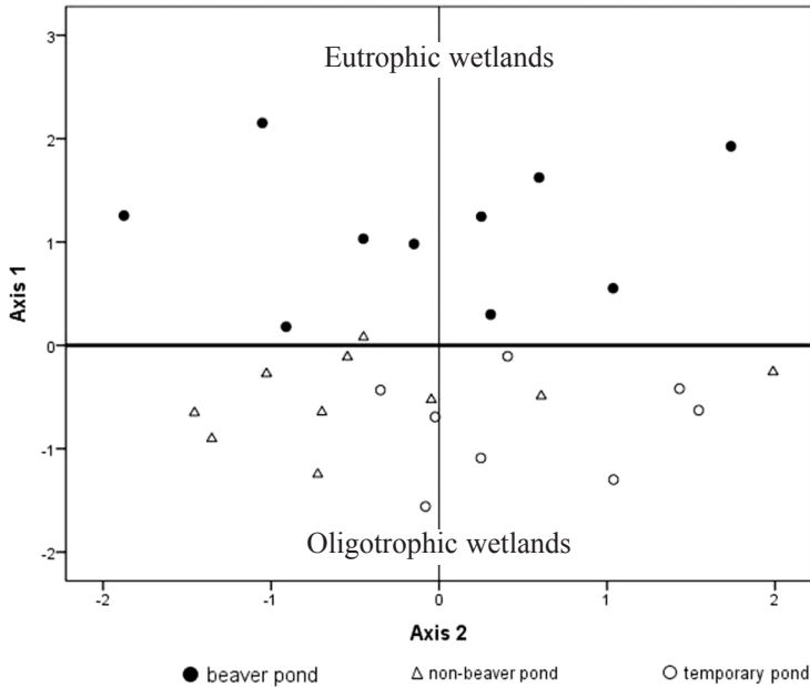
Fig. 2: The position of the 28 studied water bodies in the graphic representation of the Principal Component Analysis. Filled circles – Beaver ponds, triangles – non-beaver ponds, empty circles – temporary ponds.
