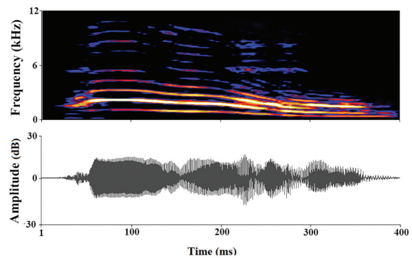
Figure 1. Spectrogram (above) and oscillogram (below) of Leptodactylus knudseni distress call (SVL: 97 mm). Puerto Gaitan, Meta Colombia (17 May 2018).
