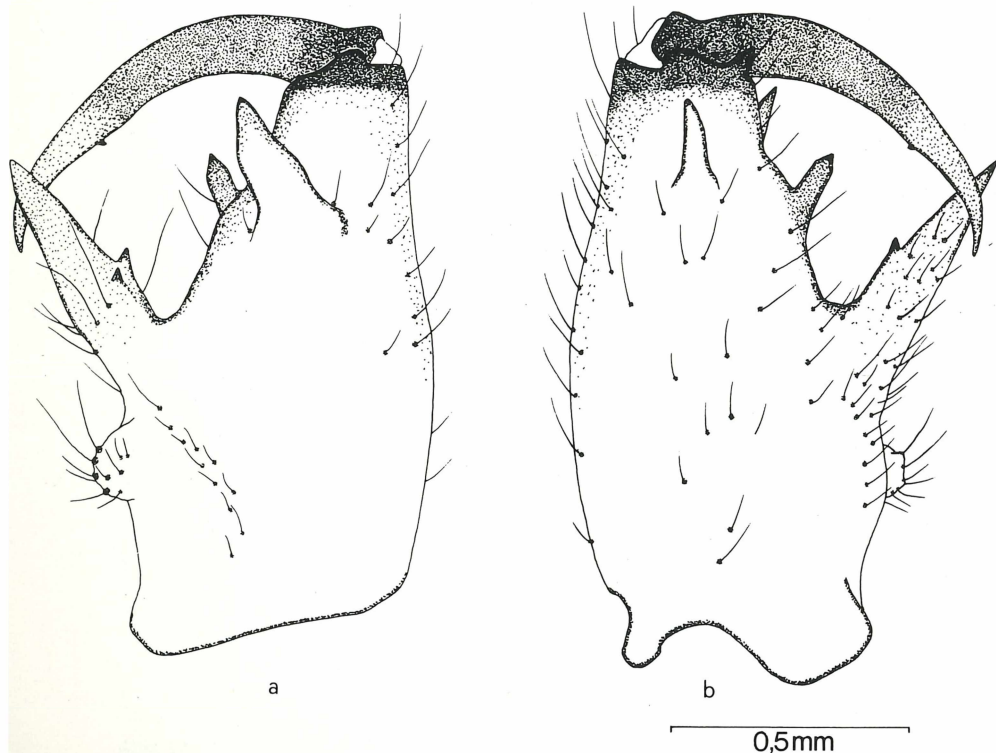
Abb. 1. Enoplognatha crucifera THORELL; linke Chelicere des ♂; a = ventral, b = dorsal.
