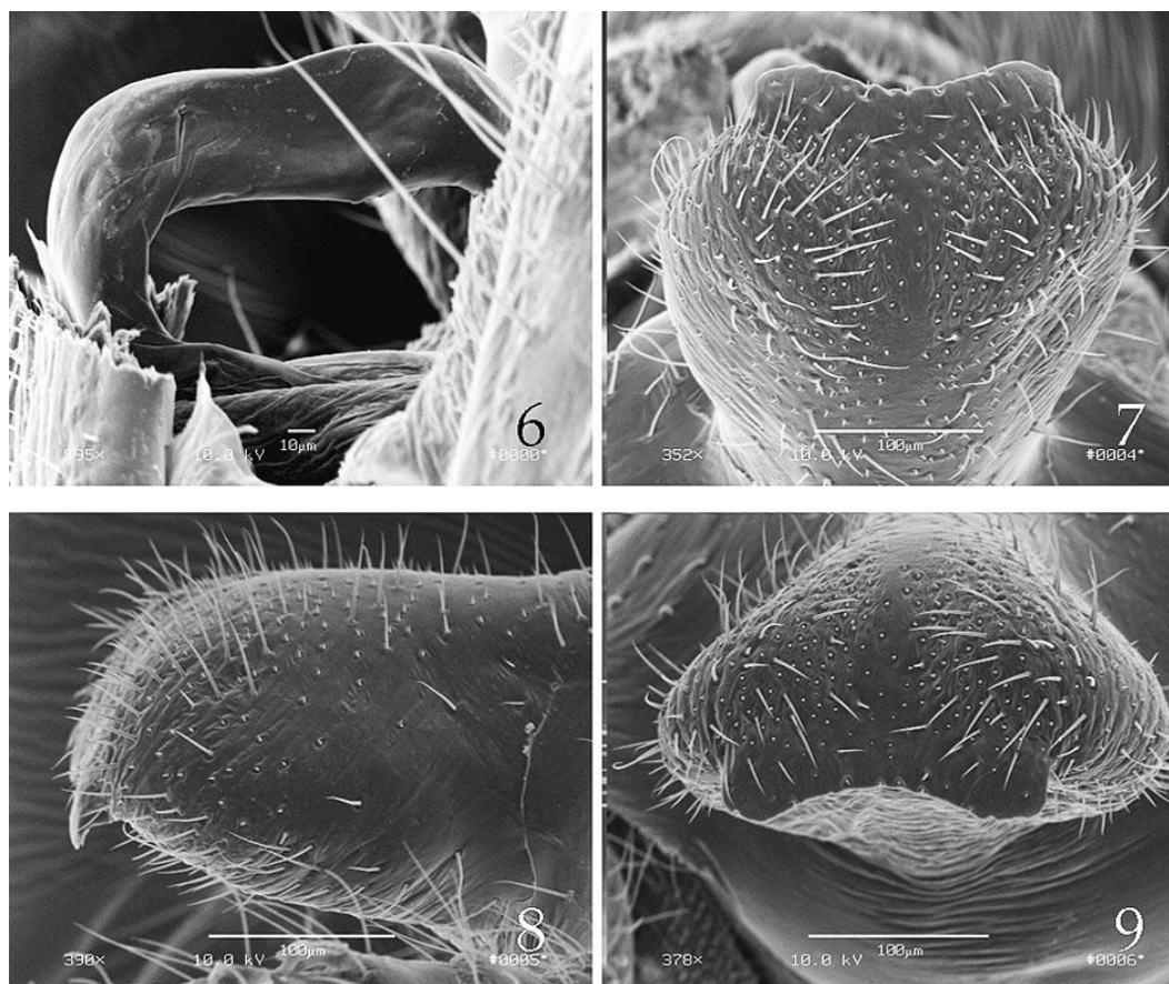
Figs. 6-9. Scanning electron micrographs of Claudioperla tigrina male genitalic structures. 6. Epiproct, lateral, apex concealed, paraprocts removed. 7. Tergum 10 process, dorsal. 8. Tergum 10 process, lateral. 9. Apex of tergum 10 process, caudal.
