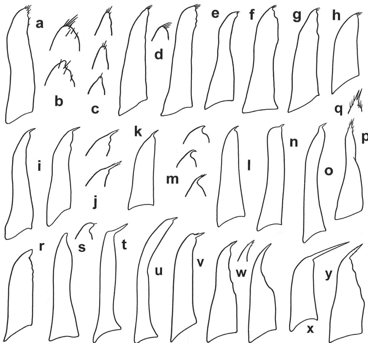
Fig. 3. Forceps type 3a, with a number of small bristles extending beyond apex (a–h); forceps type 3b, with an apical spine of stuck bristles (i–o); forcipes of intermediate evolutionary stages (p–v); forceps type 2b, with strongly sclerotized tips (w–y). a. Caenis anceps . b. Caenis anceps , different shapes of tip at higher magnification. c. Caenis hilaris , different shapes of tip. d. Caenis beskiden-sis , different shapes and tip at higher magnification. e. Caenis pseudorivulorum . f. Caenis lactea . g. Caenis picea . h. Caenis kare-nae . i. Caenis pusilla , different shapes. j. Caenis pusilla , different shapes of tip at higher magnification. k. Caenis gephyria . l. Caenis nigropunctatula . m. Caenis nigropunctatula , different shapes of tip at higher magnification. n. Caenis abdita . o. Caenis bidigitata . p. Caenis valentinae . q. Caenis valentinae , tip at higher magnification. r. Caenis ghibana . s. Caenis afrocaenoides , with different shapes of tip. t. Caenis angolensis . u. Caenis filappendices . v. Caenis nigricola . w. Caenis basuto , different shapes. x. Caenis gut-tata . y. Caenis maratha .
