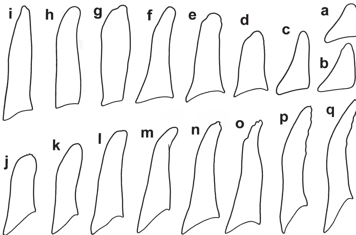
Fig. 1. Forceps type 1, apically rounded. a–c. Caenis wegneriana , different shapes. d–f. Caenis elouardi , different shapes. g. Caenis vermifera . h. Caenis obtusostilata . i. Caenis ranauensis . j. Caenis sigillata . k. Caenis reissi . l. Caenis ludicra . m. Caenis pflugfelderi . n. Caenis gonseri . o. Caenis panamensis . p–q. Caenis cubensis , different shapes.
