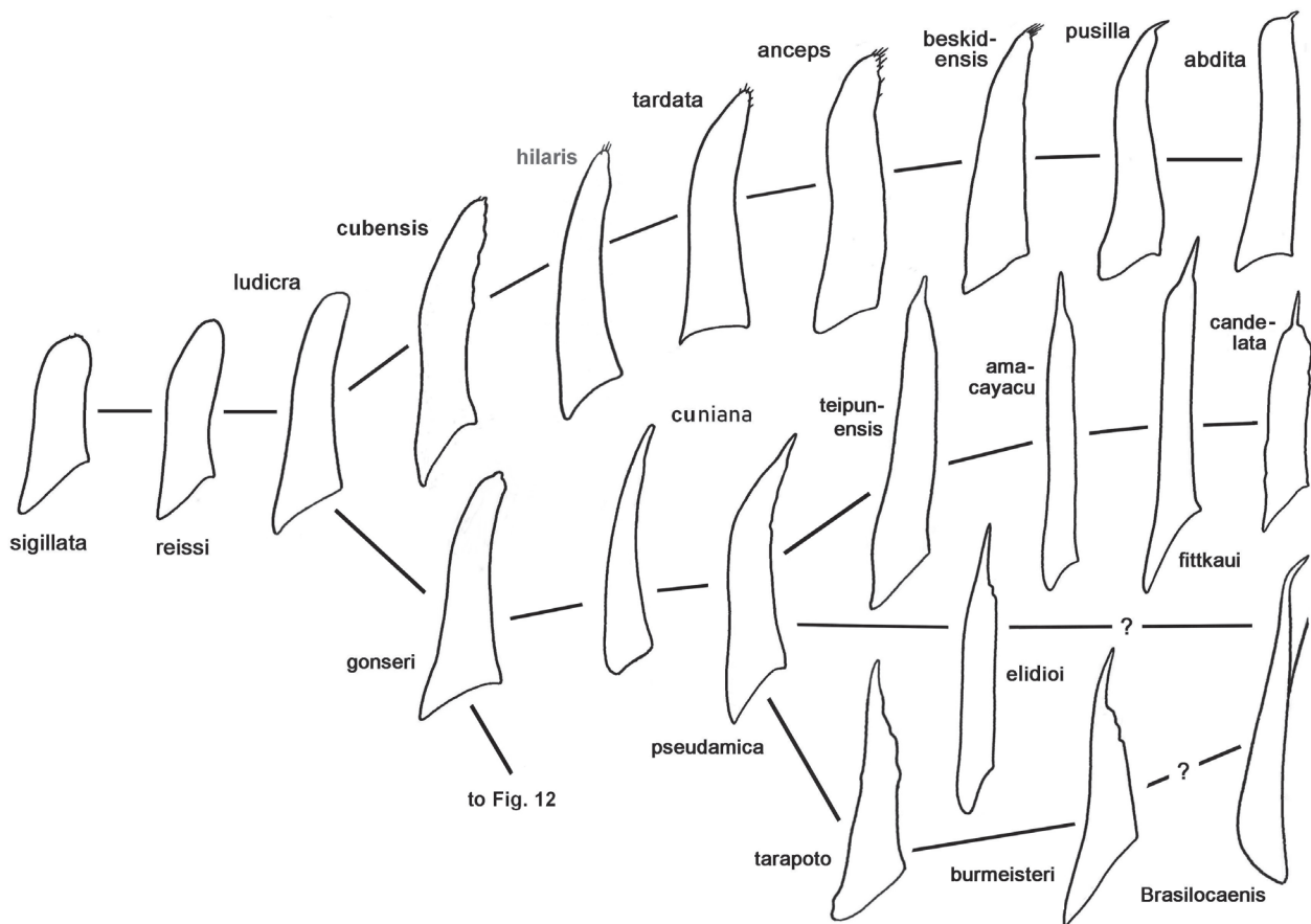
Fig. 11. Evolutionary development of forceps type 3 (upper branch) in the Nearctic, Palearctic, and Oriental realms and forceps type 2a (lower branches) in the Neotropical Realm.
