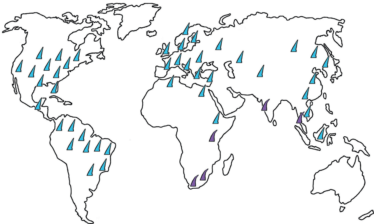
Fig. 6. Distribution of Caenis species with forceps type 2; blue: type 2a, violet: type 2b.
