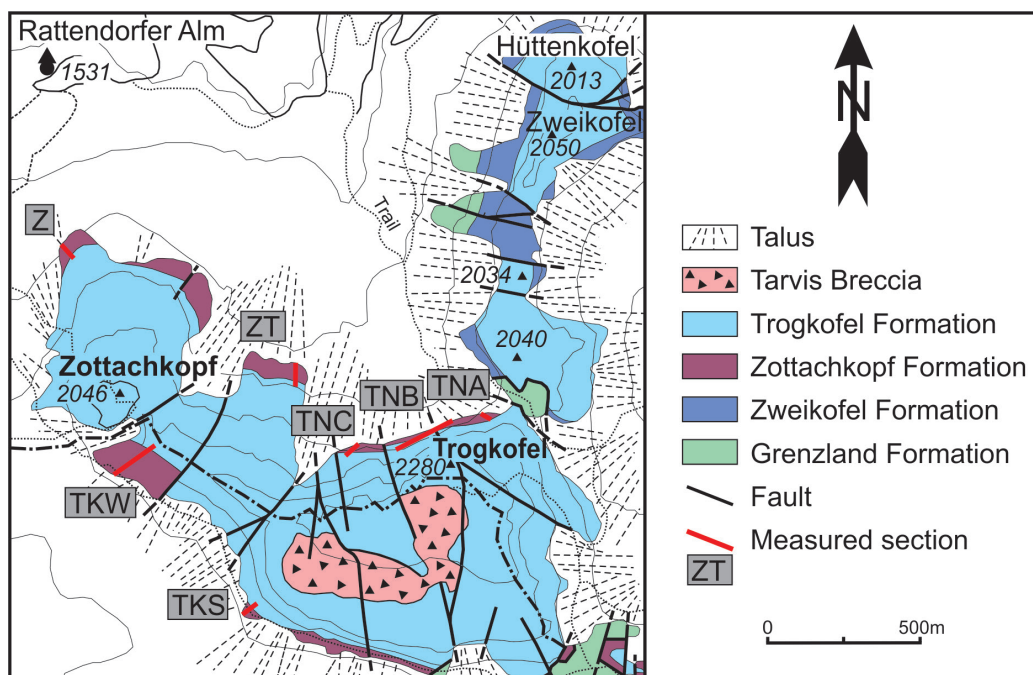
Text-Fig. 3. Simplified geologic map of the Trogkofel–Zottachkopf–Zweikofel area in the central Carnic Alps with locations of the studied sections TNA, TNB, TNC, ZT, Z, TKS and TKW.
