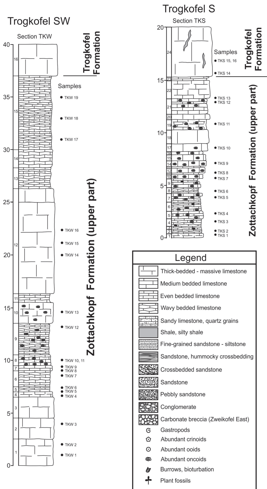
Text-Fig. 7. Lithologic sections (including legend) through the upper part of the Zottachkopf Formation and basal Trogkofel Formation at sections TKW (Trogkofel Southwest) and TKS (Trogkofel South). Locations of the sections are shown in Text-Figure 3.
