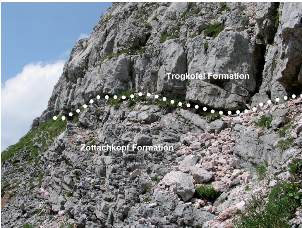
Text-Fig. 11. Bedded limestone of the uppermost Zottachkopf Formation, overlain by thick-bedded and massive limestone of the Trogkofel Formation, exposed along the trail on the southern side of Mount Trogkofel (section TKS).
