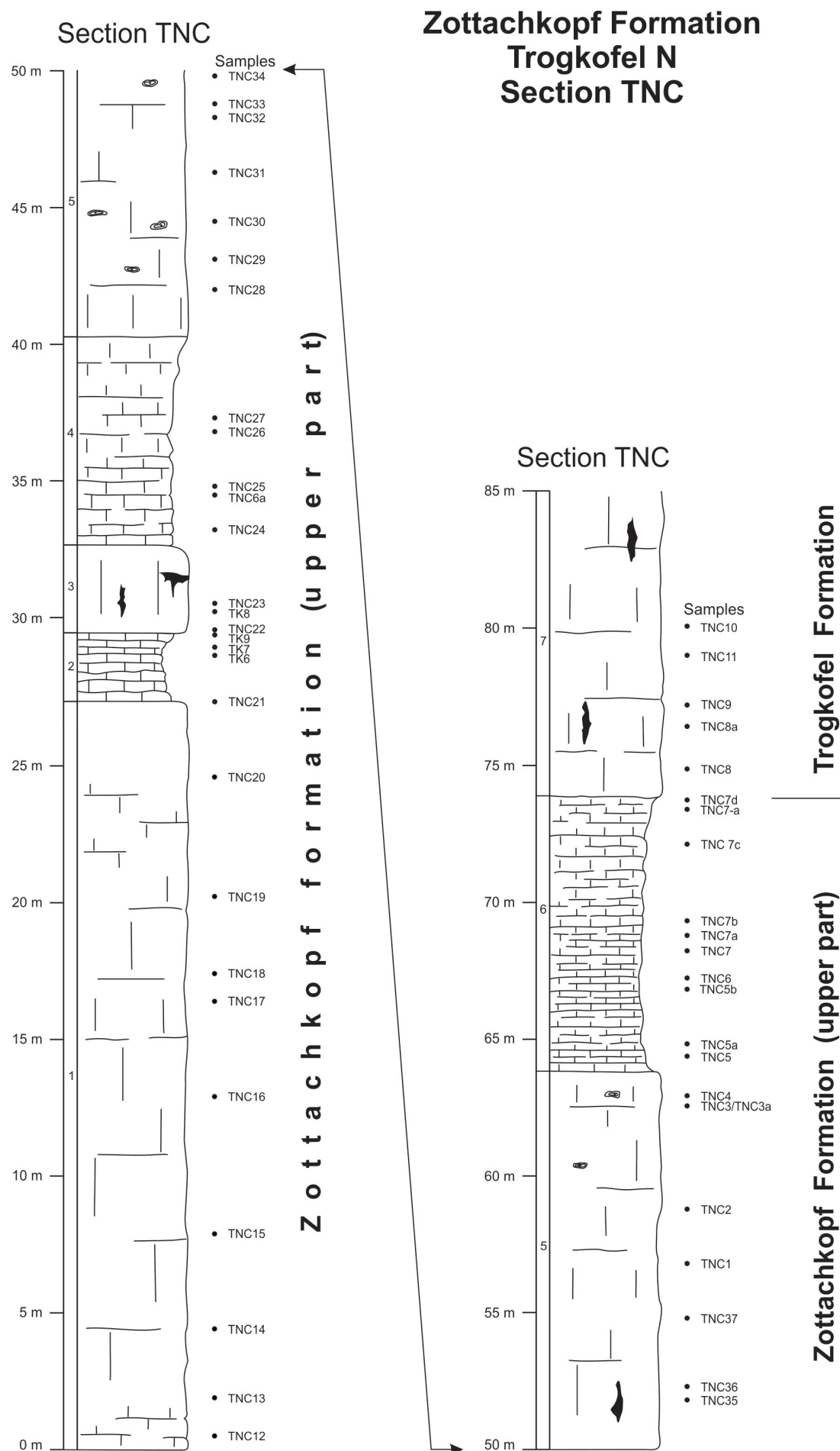
Text-Fig. 5. Lithologic section through the upper part of the Zottachkopf Formation and basal Troglkofel Formation at section TNC (Troglkofel North C) (type section). Location of the section is shown in Text-Figure 3. Legend is shown in Text-Figure 7.
