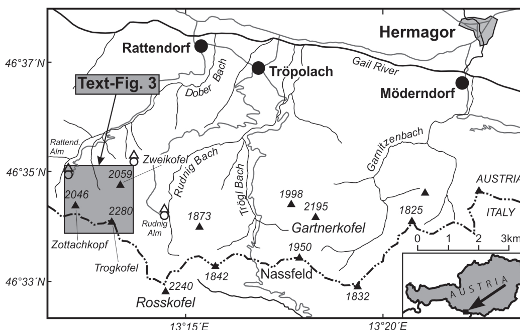
Text-Fig. 2. Map showing location of the study area in the Trogkofel-Zottachkopf massif in the central Carnic Alps along the Austrian-Italian border.
