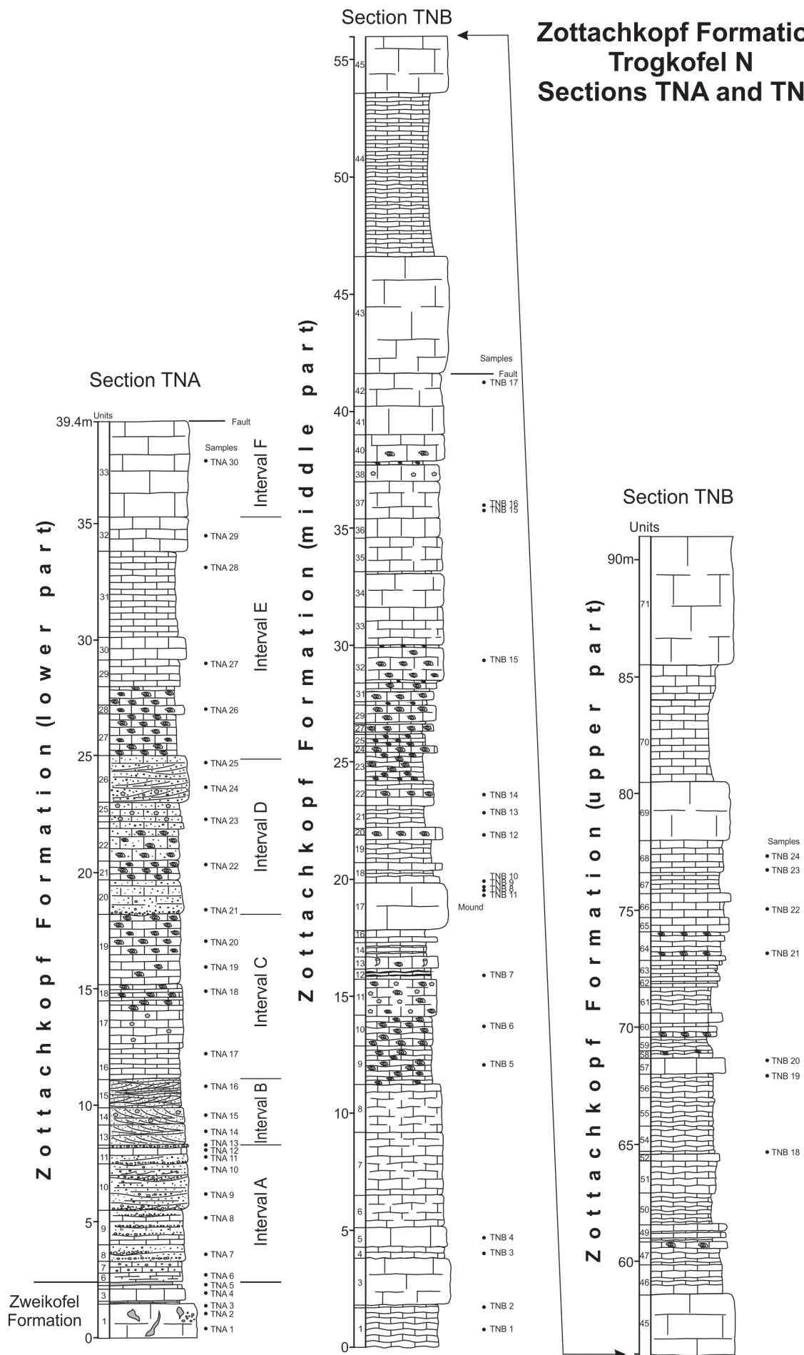
Text-Fig. 4. Lithologic section through the Zottachkopf Formation at section TNA (Trogkofel North A; lower part), TNB (Trogkofel North B; middle-upper part) (type section). Location of the sections is shown in Text-Figure 3. Legend is shown in Text-Figure 7.
