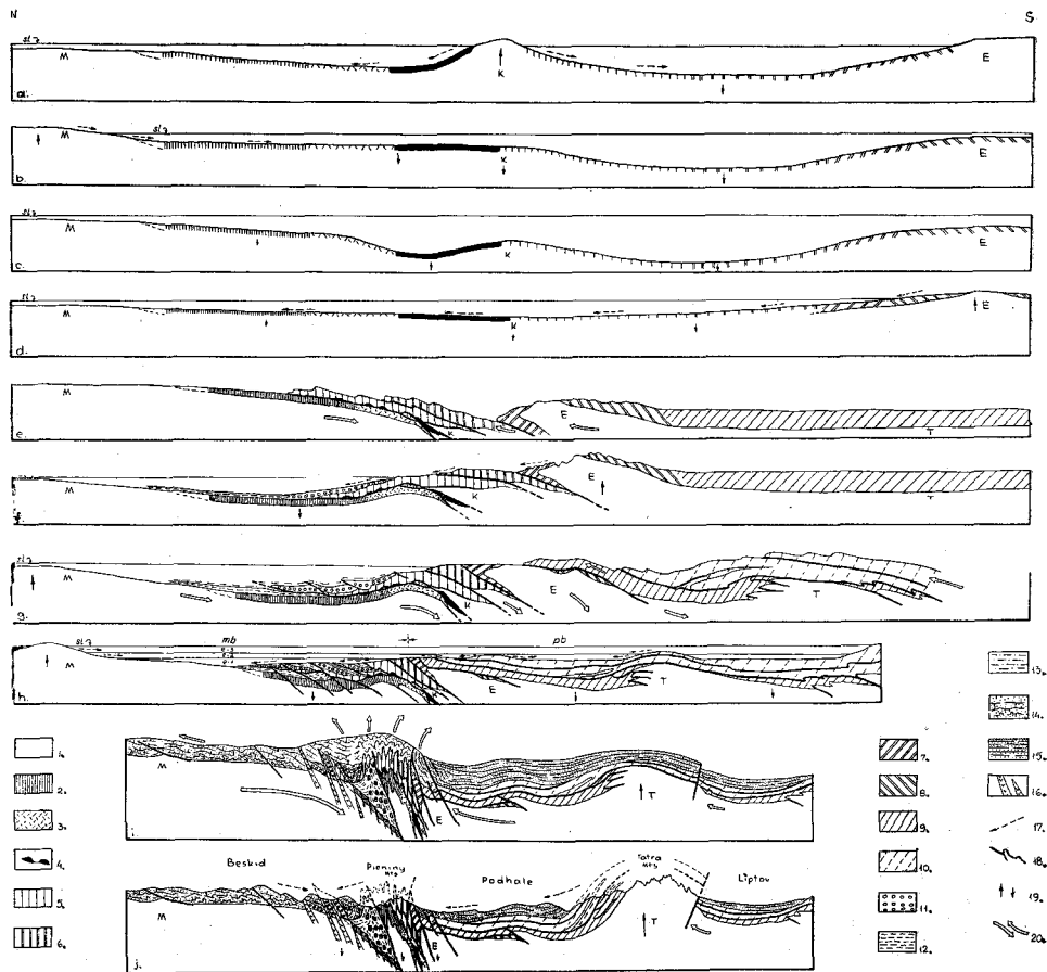
Fig. 5: Origin of the Pieniny Klippen Belt (after K. BIRKENMAJER, 1958 d, modified). Schematic presentation for the Pieniny Mts. sector. Vertical scale exaggerated. 1 = Pre-Jurassic basement rocks (in the region of the High-Tatra Series — Pre-Triassic basement rocks), 2 = Czorsztyn Series, 3 = Czertezik Series, 4 = Niedzica Series, 5 = Branisko Series, 6 = Pieniny Series, 7 = Haligowce Series, 8 = Exotic Series, 9 = High-Tatra Series ( sensu lato ), 10 = Sub-Tatra tectonic units, 11 = Jarmuta Beds (Campanian-Maestrichtian) of the Pre-Laramide Mantle, 12 = Púchov Marls (Campanian-Maestrichtian) of the Pre-Laramide Mantle, 13 = Variegated Beds (? Danian) of the Pre-Laramide Mantle, 14 = Magura Palaeogene (Post-Laramide Mantle), 15 = Podhale Palaeogene (Post-Laramide Mantle), 16 = Andesitic intrusions, 17 = direction of supply of elastics to sedimentary basins, 18 = Main tectonic contacts (overthrusts, faults), 19 = direction of the vertical movements, 20 = direction of the orogenic movements. M = Crystalline and sedimentary (Pre-Cretaceous) basement complex of the Magura Series, K = Central Cordillera in the Klippen Series basin, E = Exotic Massif (Crystalline basement and Triassic covering), T = Crystalline basement complex of the High-Tatra Series ( sensu lato ), mb = sedimentary basin of the Magura Palaeogene (e-1 = Upper Paleocene and Lower Eocene, e-2 = Middle Eocene, e-3 = Upper Eocene and Oligocene), pb = sedimentary basin of the Podhale Palaeogene, sl = sea level, a = Lower Aalenian stage, b = Bajocian stage, c = Oxfordian stage, d = Upper Turonian stage, e = Sub-Hercynian phase (Upper Coniacian-Lower Santonian) stage, f = Campanian-Maestrichtian stage, g = Early stage of the Laramide phase (Lower Paleocene), h = Upper Paleocene-Oligocene stage, i = Savian phase (Oligocene-Aquitania) stage, j = Upper Miocene-Pliocene stage.
