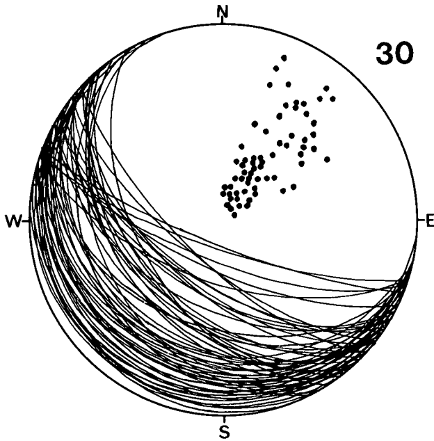
Diagramm 30: Erzberg-Nord: Hachelnock – Lannernock – Schwandnock. Wettersteinkalk. 60 s-Flächen. \beta = NW–SE, horizontal.
