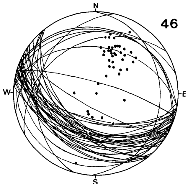
Diagramm 46: Altenberg-W und-SW. Wettersteinkalk, Raibler Schichten, Hauptdolomit. 45 s-Flächen. \beta = B = 280^\circ 6' \text{W} ; \beta = 286^\circ 10' - 20^\circ \text{W} ; \beta = B = 300^\circ 5' \text{NW} ; \beta = 346^\circ 36' \text{N} .
