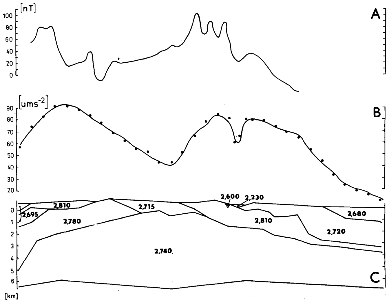
Fig. 4. Geophysical data and resulting density model of the Desná dome.
