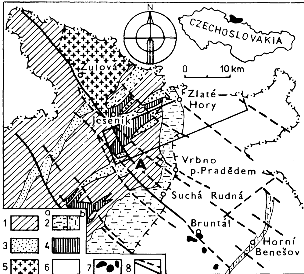
Fig. 1. Geological setting of the area studied.
