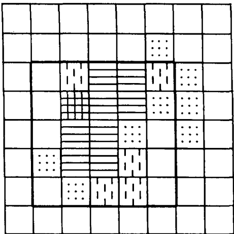
8903 (n = 101) Tonalitporphyrit
