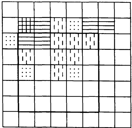
9790 (n = 101) Mikrogranitporphyr
