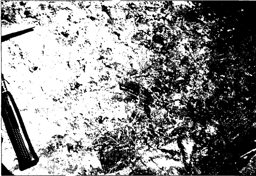
Fig. 12. Poorly sorted, clast-supported amphibolite breccia composed of different types of angular amphibolite clasts and a few carbonate clasts.
