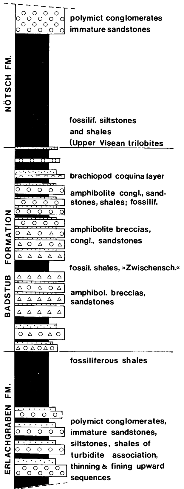
Fig. 3. Simplified stratigraphic section of the Carboniferous of Nötsch.
