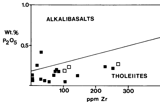
Fig. 7. P 2 O 5 vs. Zr plot (after WINCHESTER & FLOYD 1976). Symbols as in Fig. 6.
