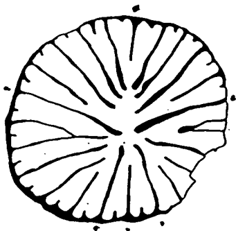
Abb. 19. Ufimia tricyclica SCHINDEWOLF, 1942? 65 AR 44/2, 2,1x.
