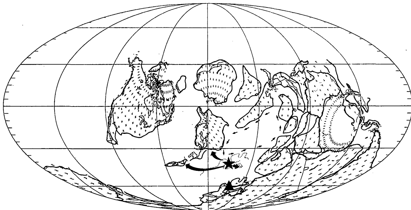
Fig. 6. Latest Ordovician (Ashgillian) paleogeography. Triangle indicates position of Southern Alps according to C.R. SCOTESE & W.S. MCKERROW (1990). The author's latitudinal setting is indicated by the star. Faunal relationships are shown by thick arrows and oceanic circulation system in the southern mid-European ocean by small arrows. Modified from C.R. SCOTESE & W.S. MCKERROW (1990).
