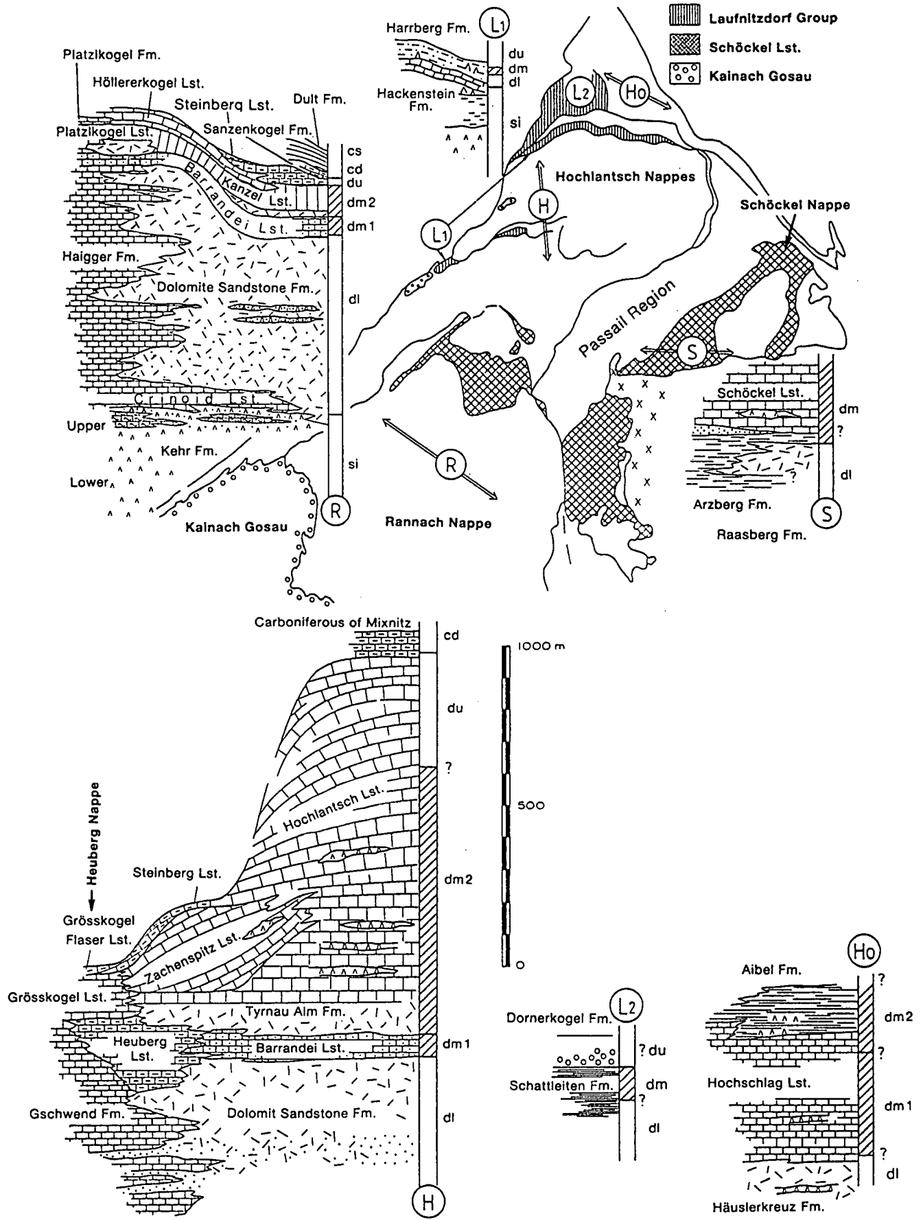
Fig. 12. Stratigraphy of the Paleozoic sequences in the surroundings of Graz. After H.W. FLÜGEL & F. NEUBAUER (1984). L 1 , L 2 = Laufnitzdorf Group; H = Hochlantsch Group; S = Schöckel Group; si = Silurian; dl = Lower Devonian; dm = Middle Devonian; du = Upper Devonian; cd = Dinantian; cs = Silesian.
