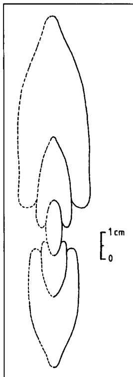
Text-Fig. 12. Bouhamidoceras sp. Cross-section of a subadult specimen. Late Hettangian – Early Sinemurian. Steinplatte II.
