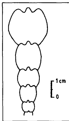
Text-Fig. 18. Paracaloceras gr. coregonense (Sow.). Cross-section of an adult specimen. Late Hettangian – Early Sinemurian. Steinplatte II.
