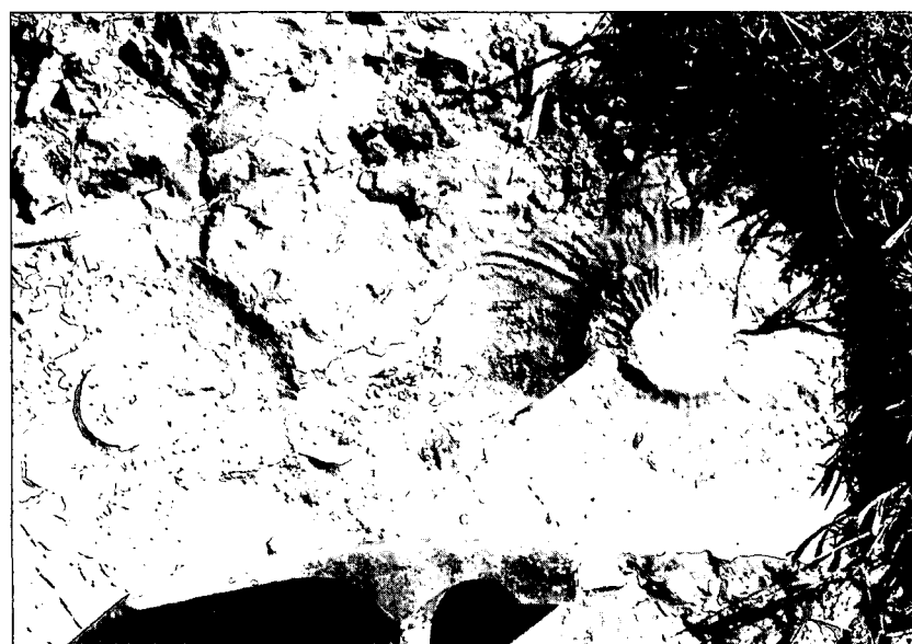
Text-Fig. 7. Surface of the same bed as Text-Fig. 6 with Angulaticeras marmoreum (Opp.).
