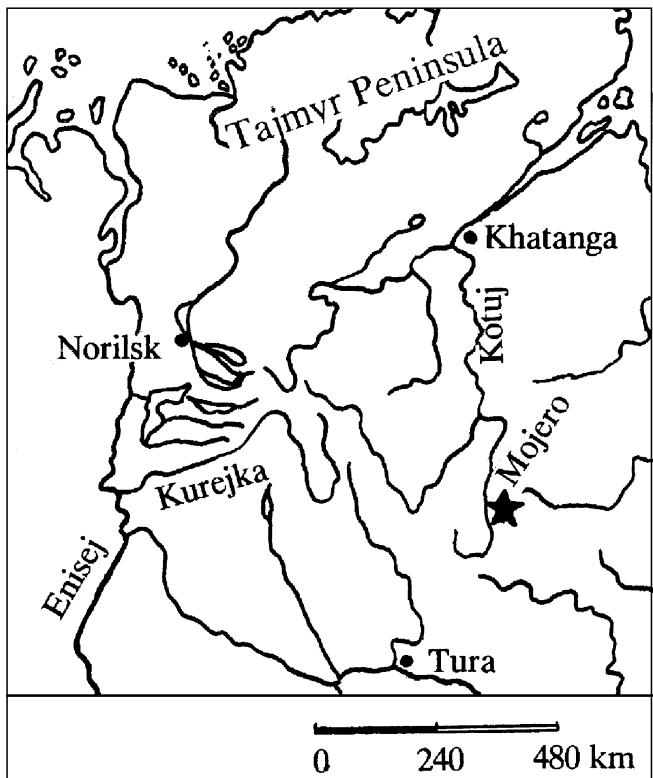
Text-Fig. 1. Locality map. Mojerokan river section marked by star.
