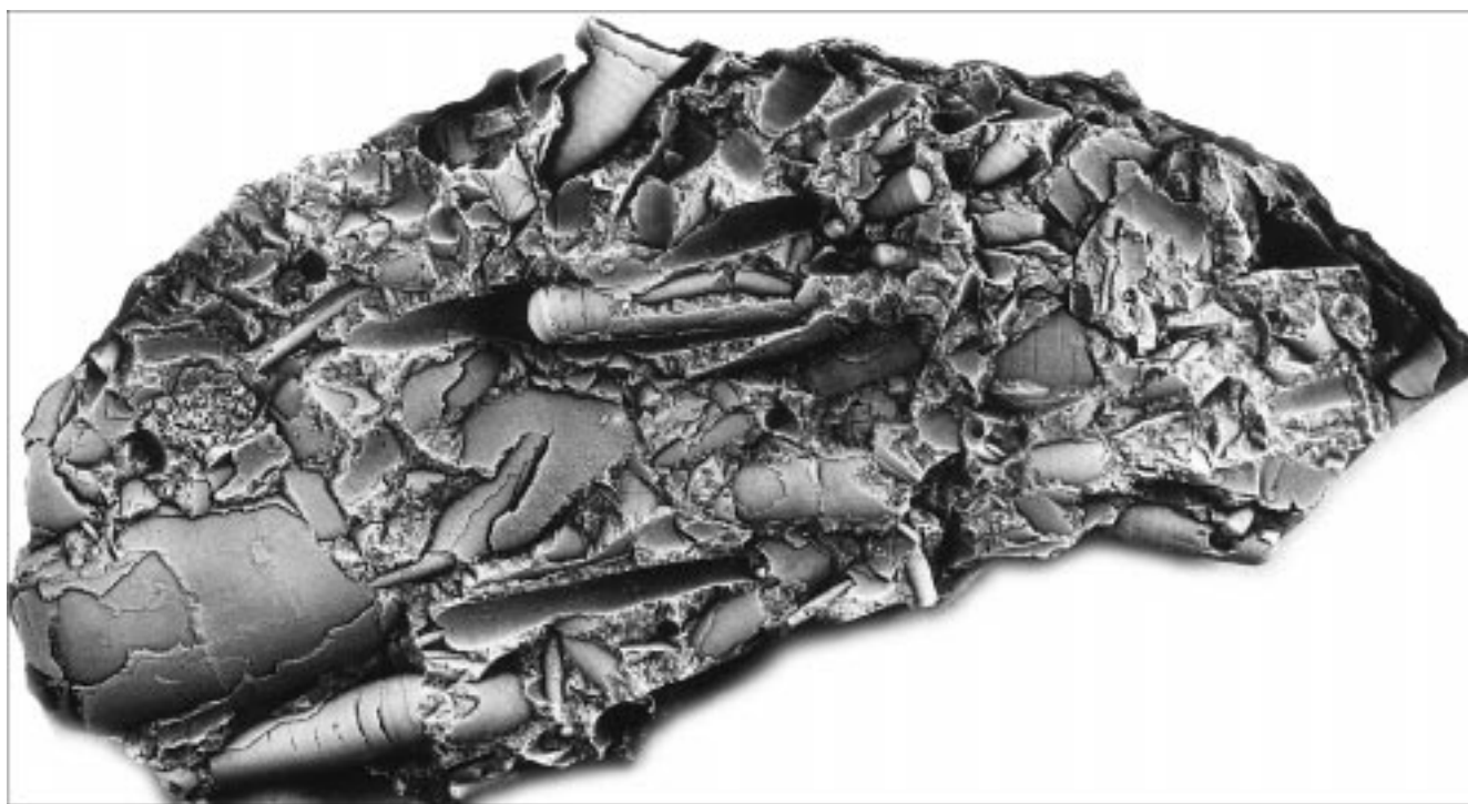
Text-Fig. 4. Lower Silurian Cephalopod limestone of the Mojero river section. Photograph by O.K. BOGOLEPOVA. Natural size.
