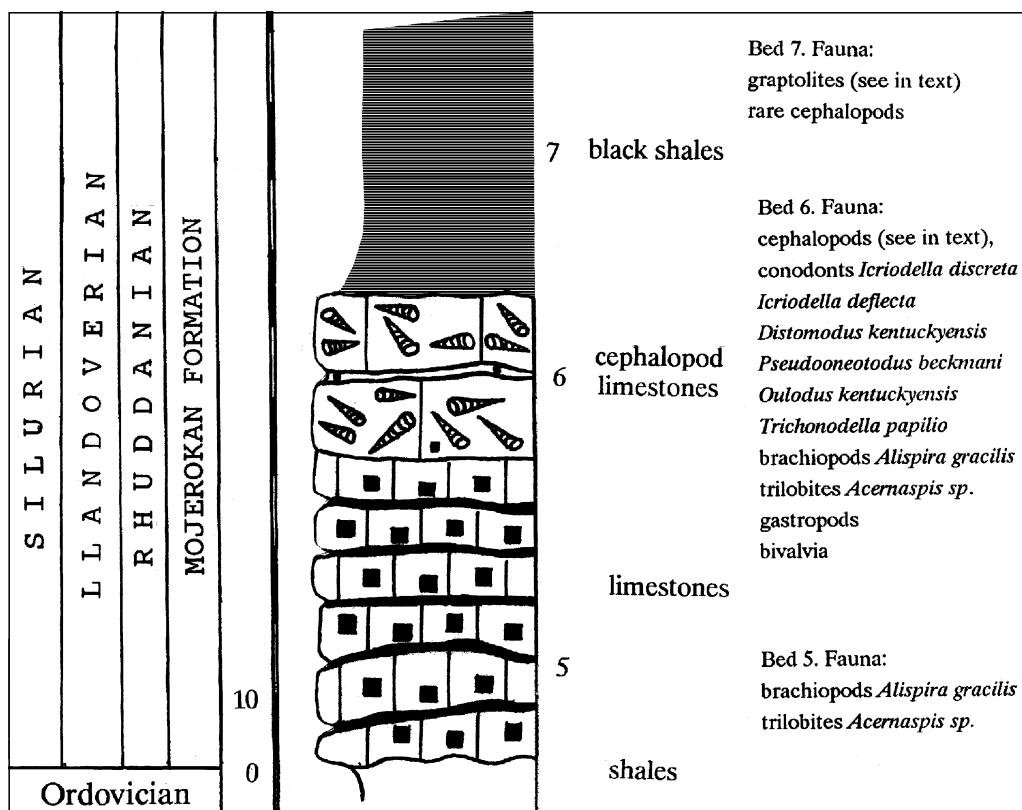
Text-Fig. 2. Lower part of the Mojerokan river section (O. BOGOLEPOVA, section OB782), showing cephalopod limestones.
