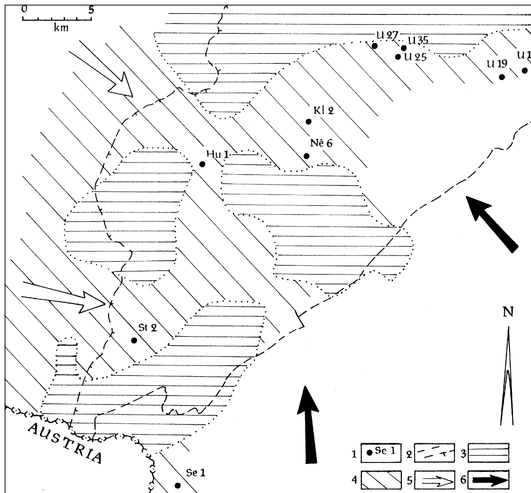
Text-Fig. 4. Palaeogeographic sketch showing distribution of the Gresten Fm in S Moravia.
