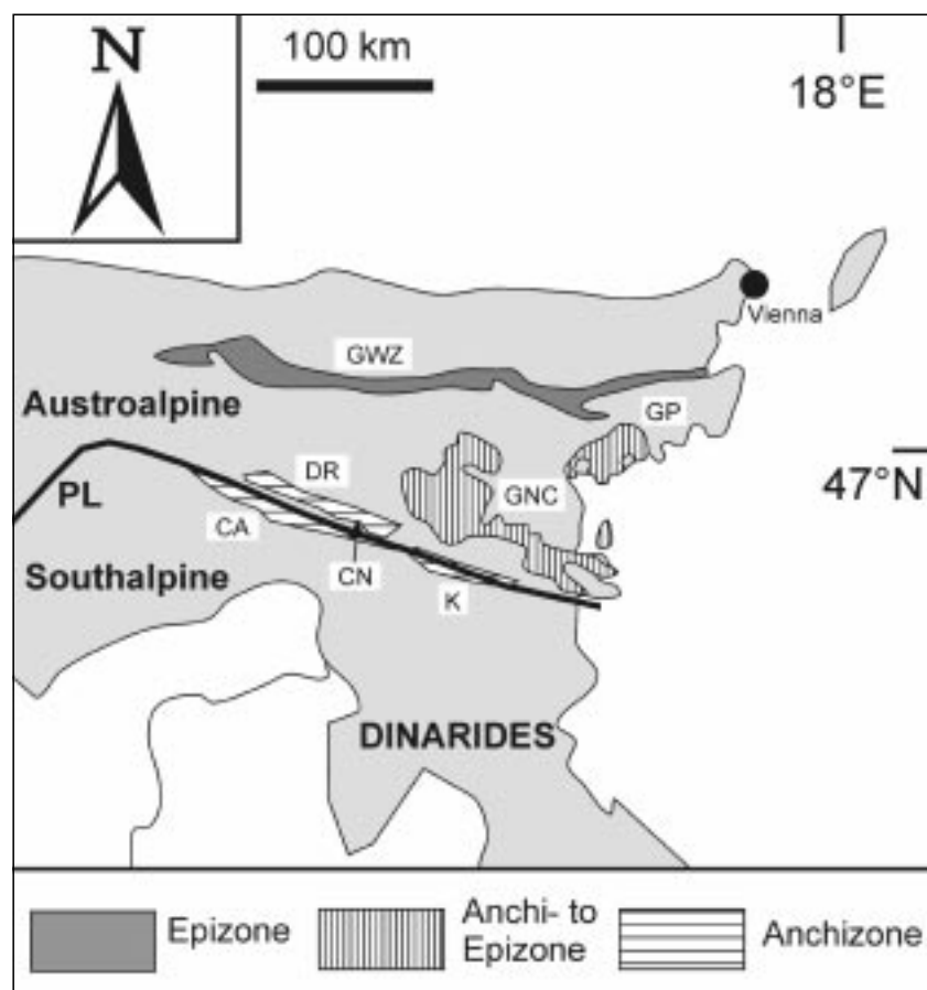
Text-Fig. 1. Location of the Gurktal Nappe Complex (GNC) within the Eastern Alps.
